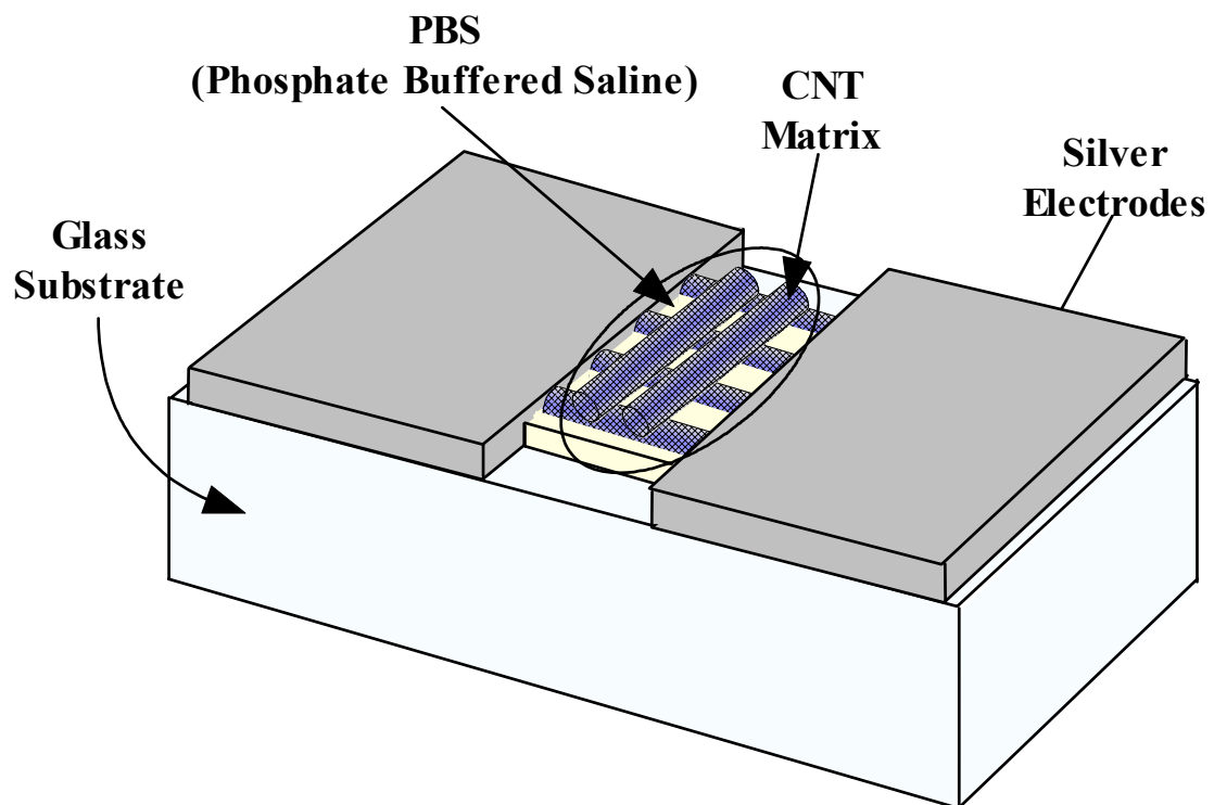
Figure 7.1: Simple SWNT conductance-based bio-sensor for detecting 10 \mu l IgG antibody [11].
