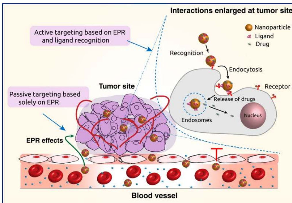
Fig. 2 Graphical illustration of passive and active drug targeting strategies. In passive targeting, the nanocarriers pass through the leaky walls and accumulate at the tumor site by the enhanced permeability and retention (EPR) effect. Active targeting can be achieved using specific ligands that bind to the receptors on the tumor cells
