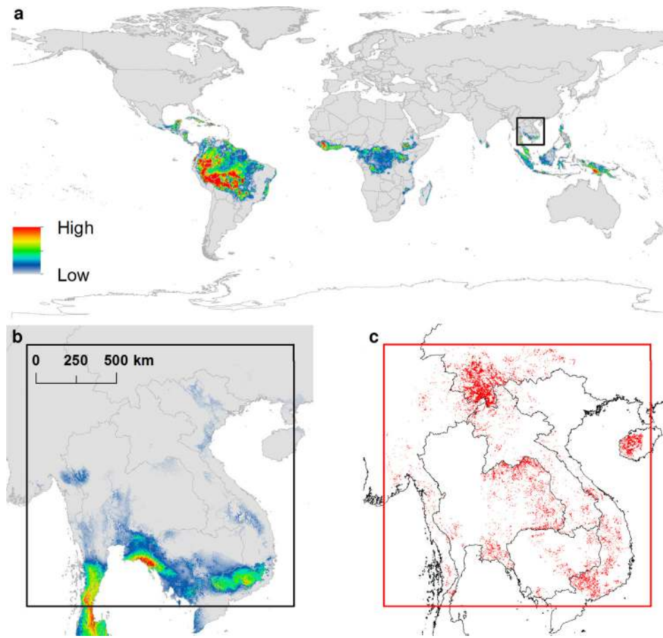
Fig. 1. Distribution of historically suitable environmental space for rubber. (a) Global distribution of historically suitable environmental space. (b) Distribution of historically suitable environments in continental SE Asia. (c) Location of the rubber plantations in the study area in 2010 (mapped at resolution of 250 m by Li and Fox (2012); map has 1 km spatial resolution for better visibility).
