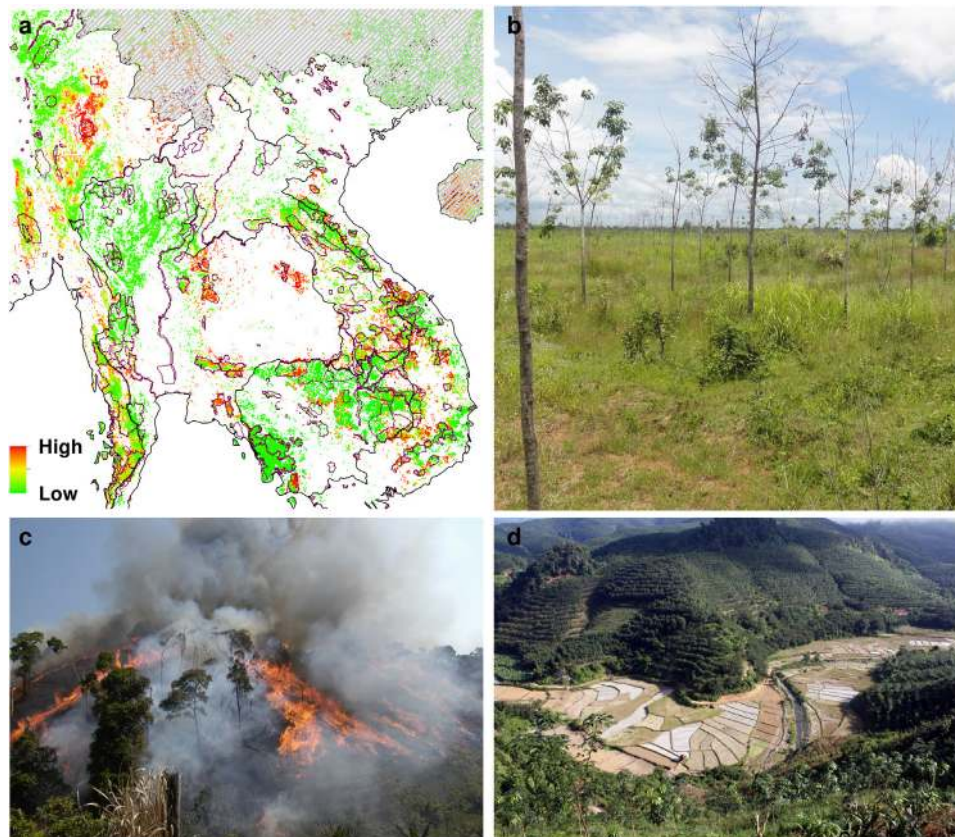
Fig. 4. Predicted conversion risks. (a) Predicted conversion risk to the remaining forests and Key Biodiversity Areas (KBAs). The KBAs are shown as purple polygons. China is greyed out as no further rubber expansion targets are known for this country. (b) Failed rubber plantation in southern Laos near the Cambodian border. (c and d) Rubber plantations are rapidly displacing forests and shifting agriculture in Xishuangbanna, China. Twenty percent of the landscape in this prefecture has been converted to rubber plantations – partly on steep slopes and altitudes >900 m.
