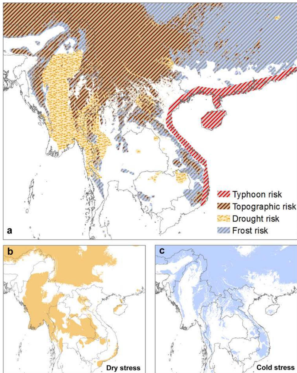
Fig. 3. Environmental stress map. (a) Areas where environmental stresses are so severe that there is a risk of unsustainability. To generate a composite map of primary risks we first delineated the typhoon and topographic risk zones, and then assigned remaining risk areas to the drought zone or frost zone depending on which was furthest from its optimum (median value within the natural rubber range). (b) Sub-optimal areas with dry stress. (c) Sub-optimal areas with cold stress.
