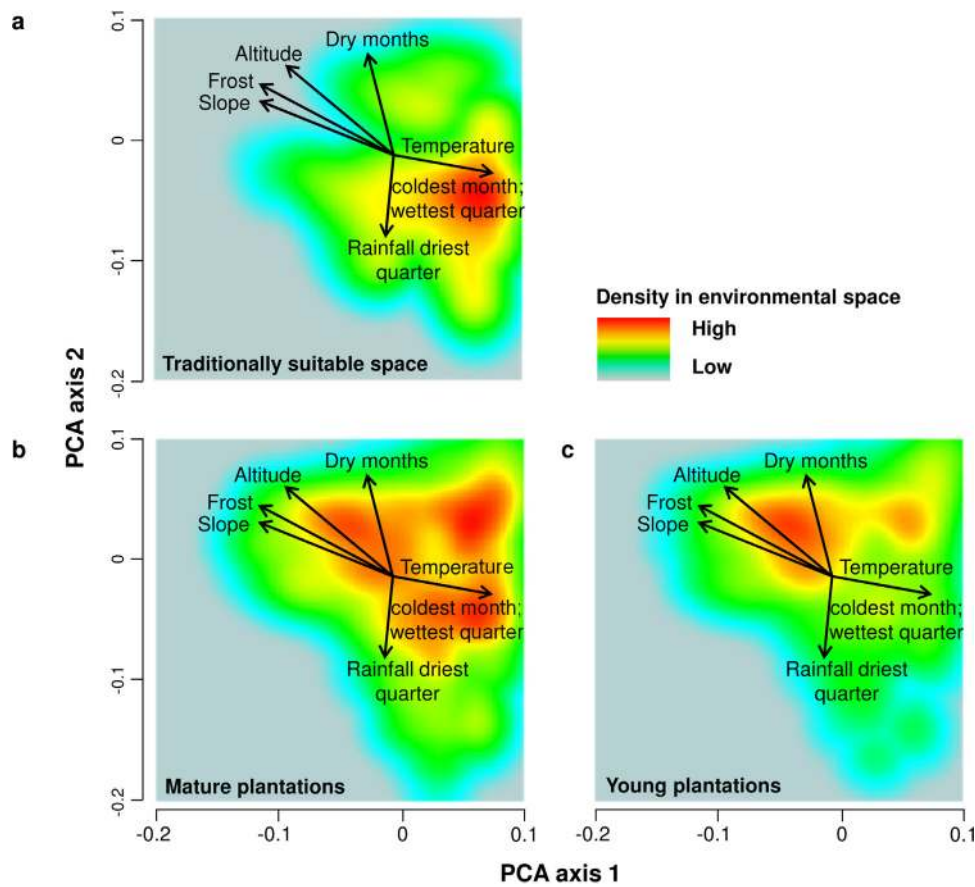
Fig. 2. Density of young and old rubber plantations in environmental space. The two-dimensional representation of environmental space was generated using a Principal Components Analysis of 15 environmental variables. The first and second axes explain 38% and 24% of the variance respectively. The PCA is centred and scaled to unit variance. Key environmental variables are shown as vectors, pointing in the direction of the gradient, with the length of the vector proportional to the variables' correlation with the ordination. For full list of correlations between the environmental variables and the first and second PCA axes see Fig. B.2. (a) Historically suitable environmental space. (b) Environmental space occupied by plantations established prior to 2005, and (c) environmental space of plantings between 2005 and 2010.
