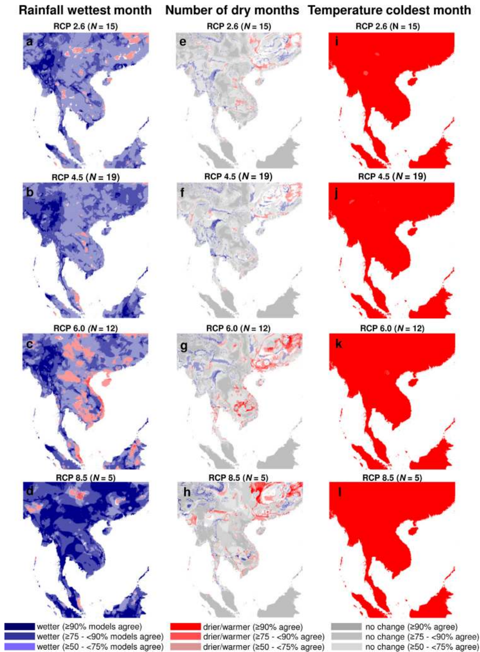
Fig. 5. Direction of climate change and model agreement across four Representative Concentration Pathways (RCPs) by 2050. The number of models included in the analysis is shown in brackets ( N ). Panels i–l show little variation as almost all models unanimously agree that temperatures in the coldest month will increase throughout the study area under all RCPs.
