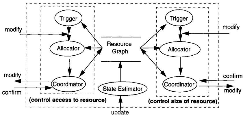
Figure 6 Functional model of a generic controller.
