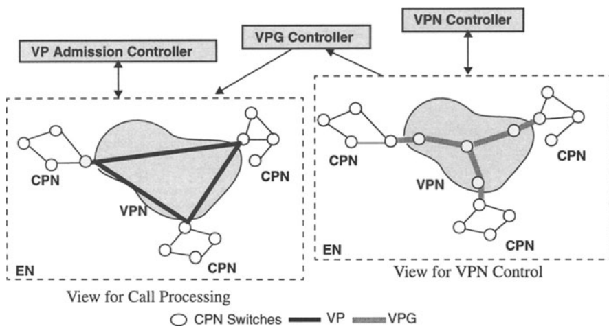
Figure 4 Network views the controllers operate on.
