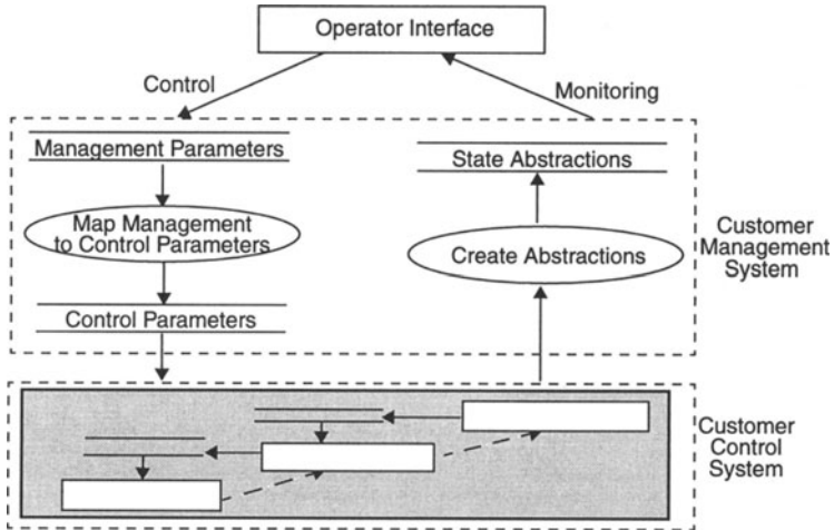
Figure 7 Framework for customer management.
