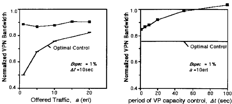
Figure 11 Performance Evaluation of the customer control system.
