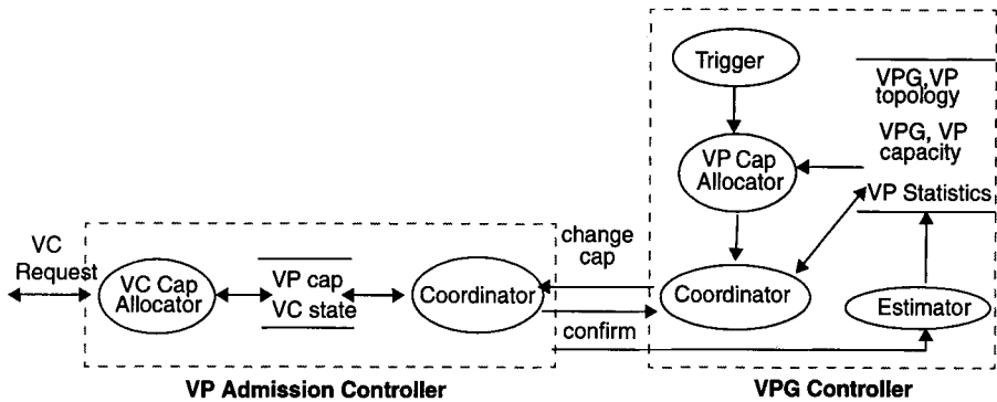
Figure 5 Functional model of a VP admission controller interacting with a VPG controller
