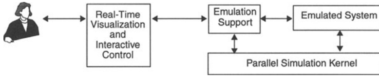
Figure 9 Building blocks of the interactive emulation platform.
