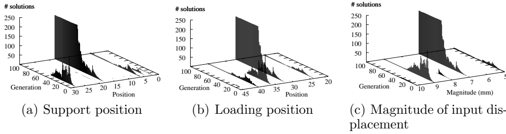
Figure 14. Evolution of applied boundary and support conditions for feasible solutions during NSGA-II run.
