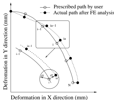
Figure 2. A prescribed path and an actual path traced by the elastic structure.
