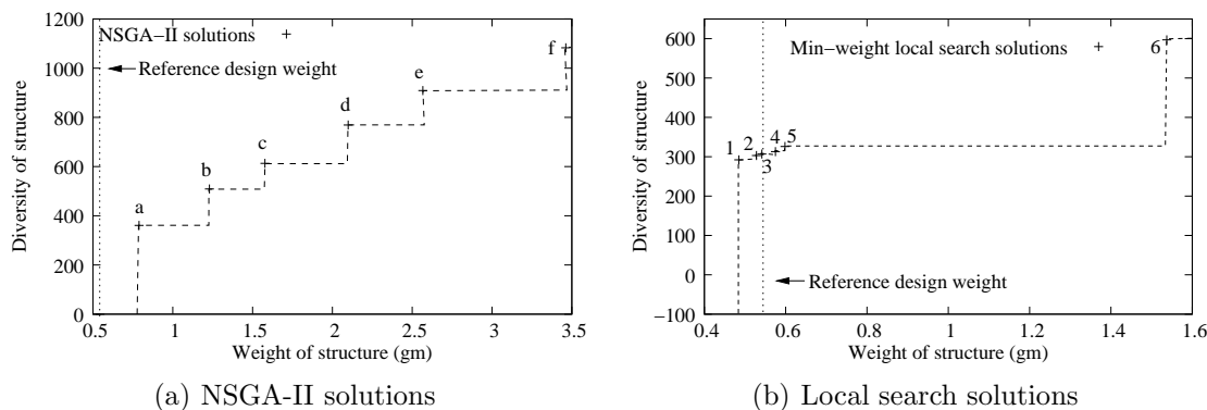
Figure 12. Bi-objective solutions for the curvilinear path tracing CMs (Example 1).
