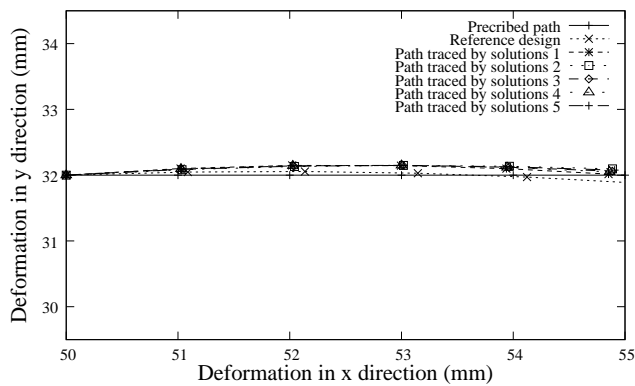
Figure 19. Prescribed path and path traced by all local search solutions.
