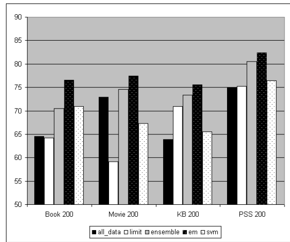
Figure 3: Accuracy with 200 labeled examples
