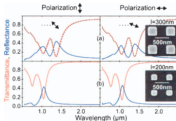
Fig. 3. Measured transmittance (red) and reflectance (blue) spectra for arrays of plate pairs. (a) w=l=300 nm, (b) w=l=200 nm. Fixed parameters: t=20 nm, d=80 nm, and a_x=a_y=l+350 nm. Orientation as in Fig. 2. Dotted curves, transmittance spectra for 45^\circ (left column) and 22.5^\circ (right column) incident polarization.
