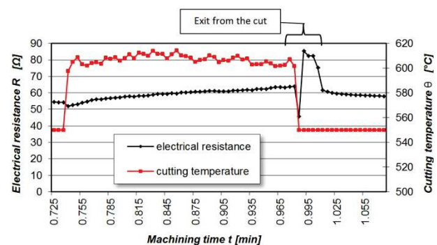
Figure 10 The dependence of electrical resistance and temperature on the machining time – record details of a cut no. 58
