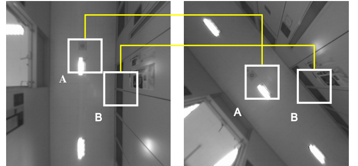
Fig. 2 Scale invariant property of ceiling image; A has rotation variation; B has rotation and shear deformation
