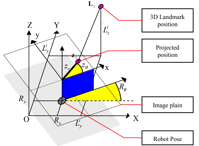
Fig. 1 Observation Model: 3D to 2D projection
