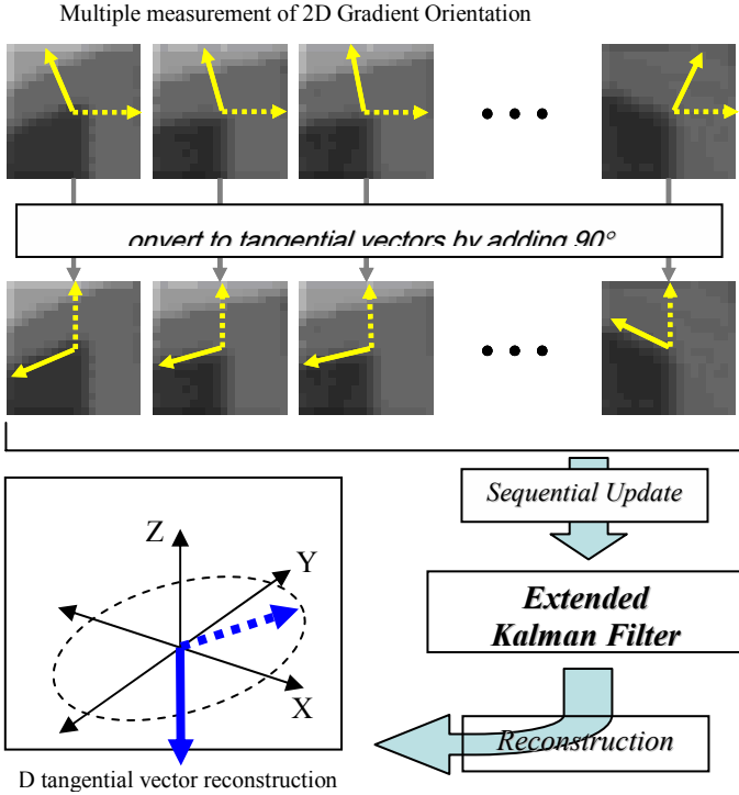
Fig. 6 3D tangential vector reconstruction using multiple 2D gradient orientation measurement
