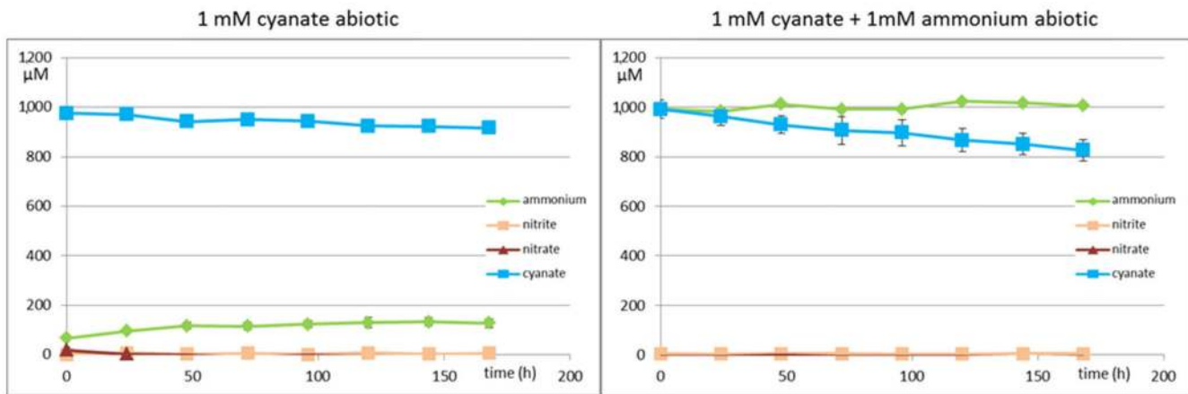
Extended Data Figure 9. Abiotic controls for the reciprocal-feeding experiment (Figure 2, Extended Data Figure 8) Concentration changes of cyanate, ammonium, nitrite, and nitrate during 168 hours incubation under similar conditions to the biotic experiments: mineral medium containing 1 mM cyanate (left) or 1 mM cyanate and 1mM ammonium (right). Cyanate decay rate is much slower than in biotic setups (see Extended Data Figure 8). Cyanate decay in the presence of ammonium led to formation of a product other than ammonium (e.g. carbamylate). No nitrite or nitrate was formed abiotically. Data points are mean values, error bars show 1 SD of three technical replicates.
