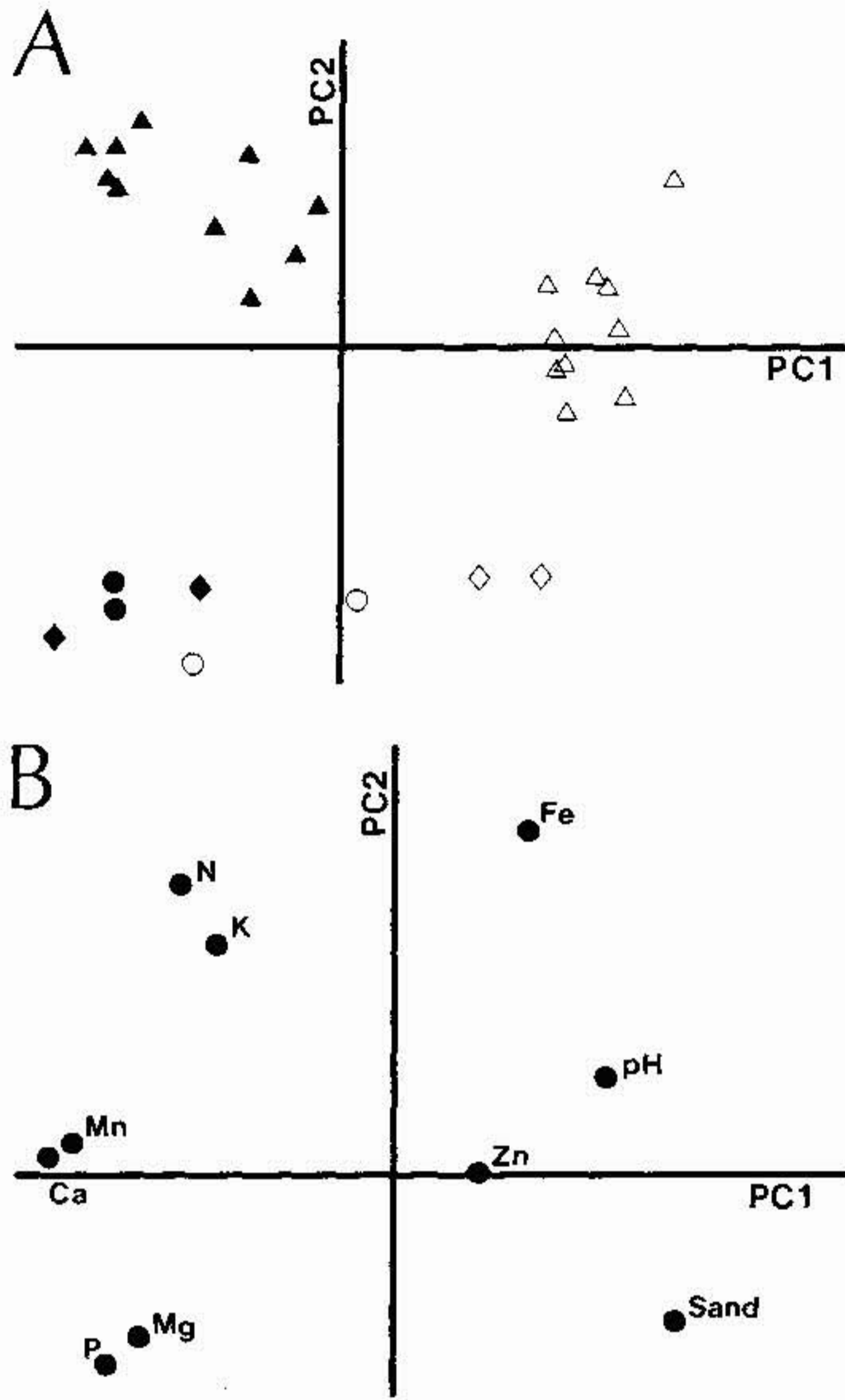
Fig. 2. A: plot of the first two components of soil samples from cryptobiotically crusted and uncrusted surfaces at three different locations (see Table 1). Samples from Arches National Park are indicated by triangles and diamonds; samples from Wind Whistle Campground are represented by circles. B: plot of weights for individual parameters used to obtain the first two components shown in Figure 2A (see text for explanation).
