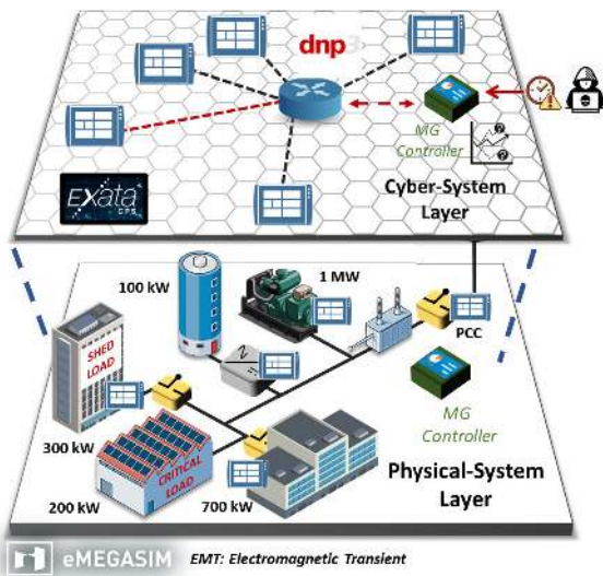
FIGURE 19. Conceptual illustration of the real-time co-simulation MG system testbed used in the TDA case study.
