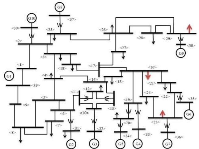
FIGURE 15. Load-changing attack on IEEE-39 bus system. Load-changing attack targets are shown as red arrows in the system topology.
