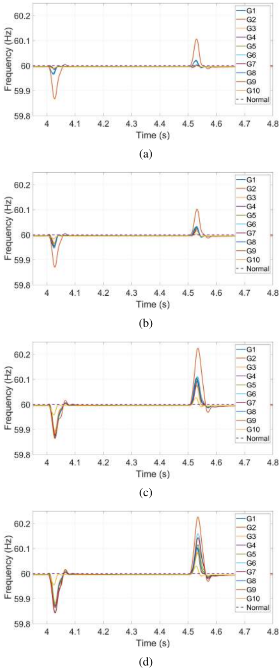
FIGURE 17. Frequency variation impact on the power grid: (a) with 20% demand increased at bus 29, (b) with 20% demand increased at buses 29 and 16, (c) with 50 % load increase at buses 29 and 16, and (d) with 50 % load increase at buses 29, 16, and 23.
