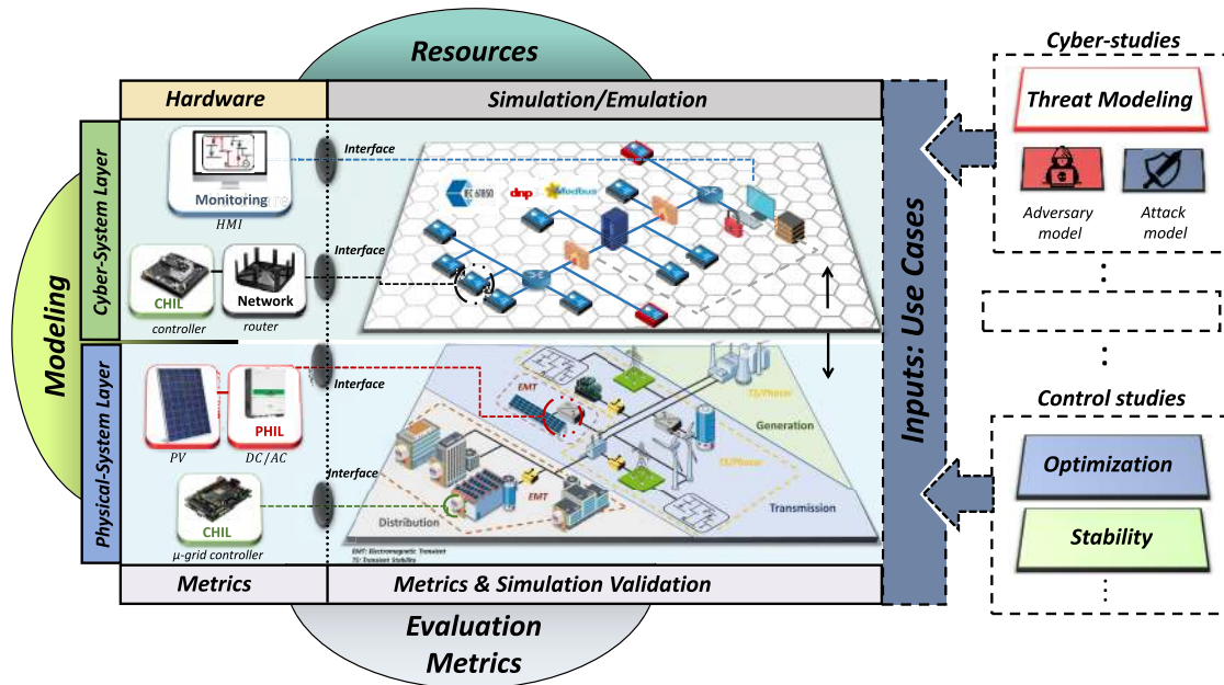
FIGURE 5. Cyber-physical system (CPS) framework: the cyber-system and physical-system layers are presented with their respective factors, i.e., modeling, resources, and evaluation metrics, needed for conducting cyber-physical studies. Different use cases requirements can be adjusted to perform CPS related investigations.
