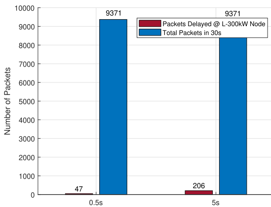
FIGURE 24. Number of packets delayed by time-delay attack (TDA) at delay = 0.5sec and delay = 5sec vs. total number of packets in 30sec.
