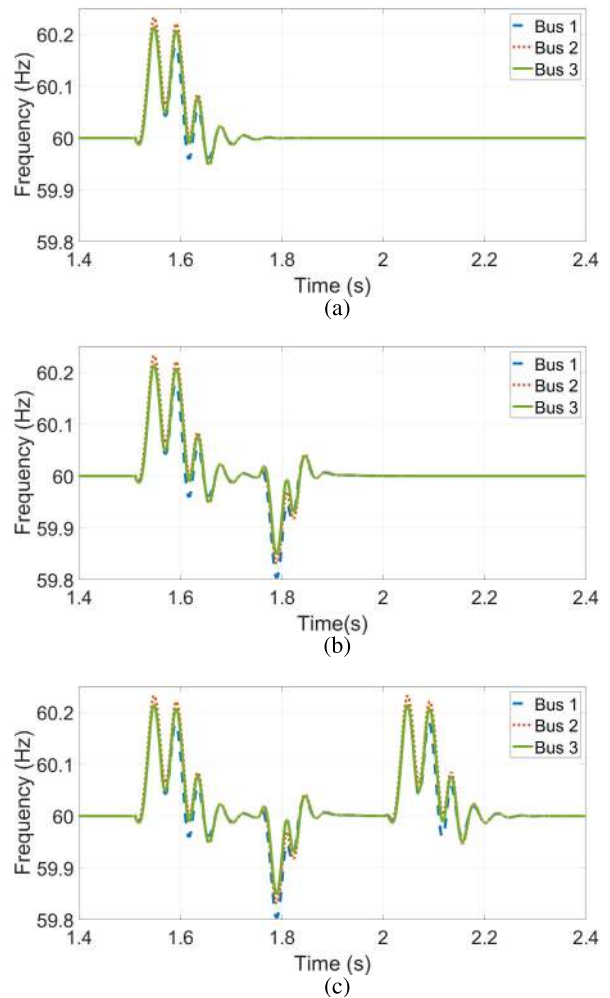
FIGURE 28. Frequency response when the CB at bus 5 of the IEEE-9 bus system is: (a) opened at t = 1.5sec , (b) opened at t = 1.5sec and then closed at t = 1.75sec , and (c) opened at t = 1.5sec , closed at t = 1.75sec , and opened again at t = 2sec .
