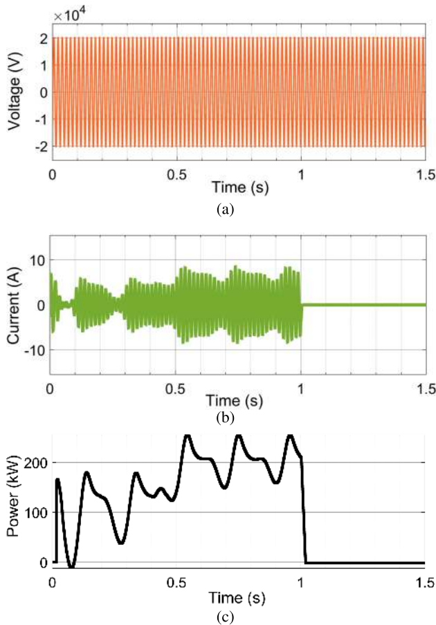
FIGURE 12. Cross-layer firmware attack impact on the DC-AC converter stage (grid-tied inverter end): (a) impact on the AC voltage output, (b) impact on the AC current output, and (c) impact on the AC power output.
