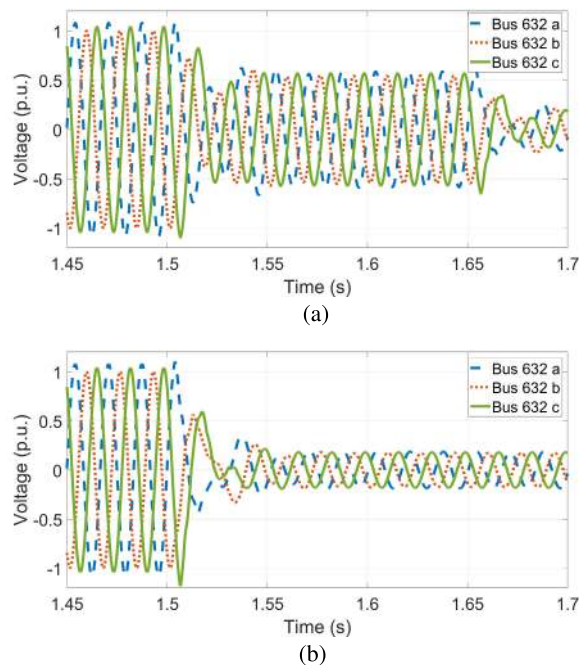
FIGURE 30. Voltage response at bus 632 (distribution system) during transmission system contingency scenarios: a) N-1-1 contingency where generators G2 is disconnected at t = 1.5\text{sec} and G3 at t = 1.6\text{sec} consecutively, and (b) N-2 contingency where generators G2 and G3 are disconnected at t = 1.5\text{sec} simultaneously.
