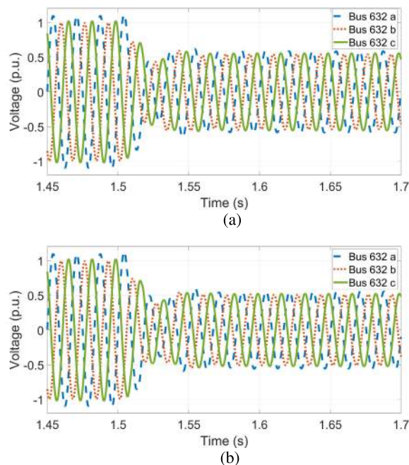
FIGURE 29. Voltage response at bus 632 (distribution system) during N-1 transmission system contingencies when: a) generator G2 is disconnected at t = 1.5\text{sec} , and (b) generator G3 is disconnected at t = 1.5\text{sec} .
