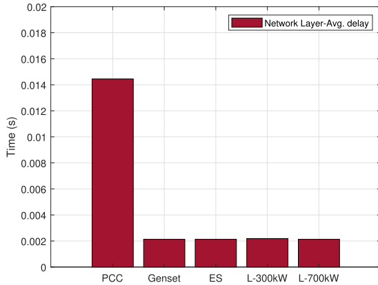
FIGURE 23. Average end-to-end delay of all nodes in the communication network (cyber layer).
