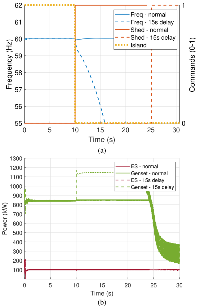
FIGURE 22. Normal operation Vs. 15sec time-delay attack (TDA) scenario: (a) EPS frequency response during a 15sec time-delay attack (TDA) on the islanding command, and (b) generator power fluctuation during the 15sec time-delay attack (TDA).
