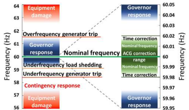
FIGURE 18. Power system corrective mechanisms to maintain stability under different frequency deviations.
