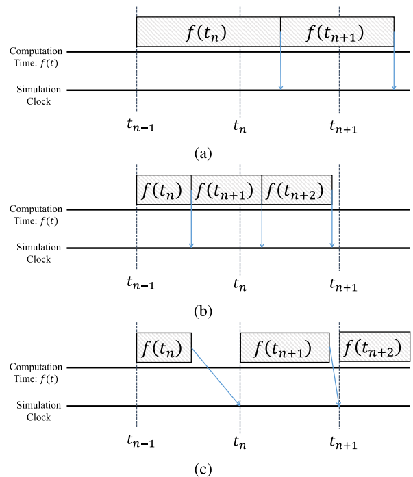
FIGURE 7. Differences in the computation timing of offline simulation and real-time simulation: (a) slower-than real-time, (b) faster-than real-time, and (c) real-time simulation.
