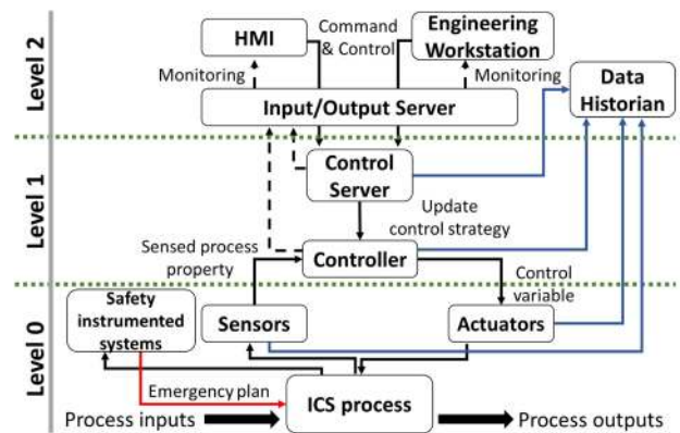
FIGURE 4. CPS functional attack levels and assets overview.
