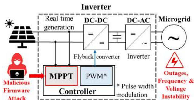
FIGURE 10. Cross-layer firmware attack targeting the inverter’s maximum power point tracking (MPPT) controller.
