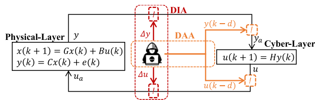
FIGURE 8. Diagram of CPS plant under DIA and DAA scenarios.
