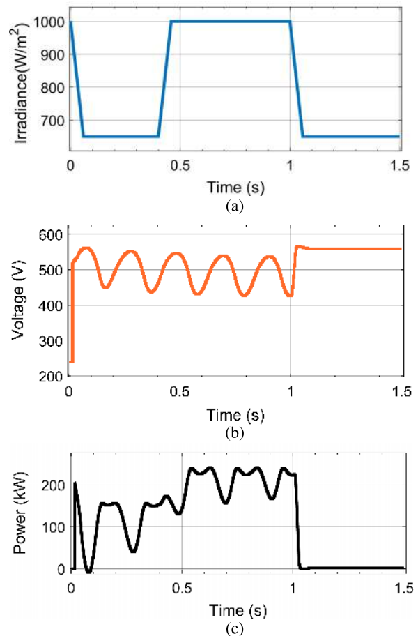
FIGURE 11. Cross-layer firmware attack impact on the DC-DC converter stage: (a) solar irradiance profile, (b) impact on the DC voltage output, and (c) impact on the DC power output.
