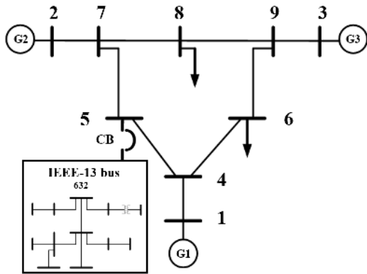
FIGURE 27. The integrated T&D real-time simulation model: it includes the IEEE-9 bus system (transmission model) and IEEE-13 bus system (distribution model).
