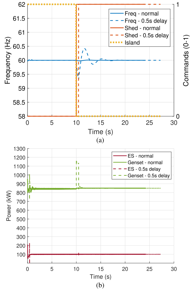
FIGURE 20. Normal operation Vs. 0.5sec time-delay attack (TDA) scenario: (a) EPS frequency response during a 0.5sec time-delay attack (TDA) on the islanding command, and (b) generator power fluctuation during the 0.5sec time-delay attack (TDA).
