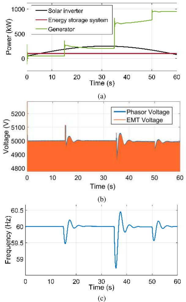
FIGURE 13. Cross-layer firmware attack impact on the power grid: (a) renewable source generated power, (b) phasor and EMT magnitude of the MG voltage, and (c) MG operating frequency.
