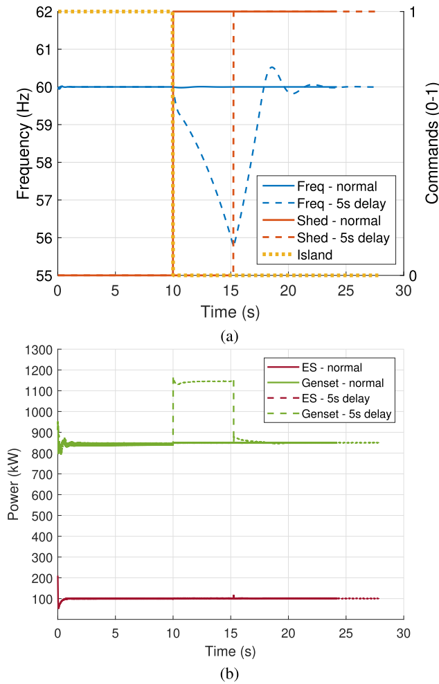
FIGURE 21. Normal operation Vs. 5sec time-delay attack (TDA) scenario: (a) EPS frequency response during a 5sec time-delay attack (TDA) on the islanding command, and (b) generator power fluctuation during the 5sec time-delay attack (TDA).
