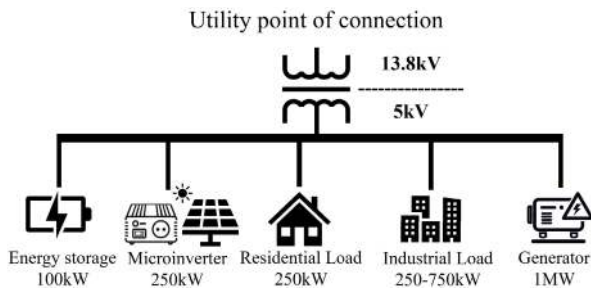
FIGURE 9. Conceptual illustration of the MG system used for the cross-layer firmware case study.
