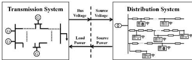
FIGURE 26. Transmission and distribution (T&D) integrated simulation system setup.
