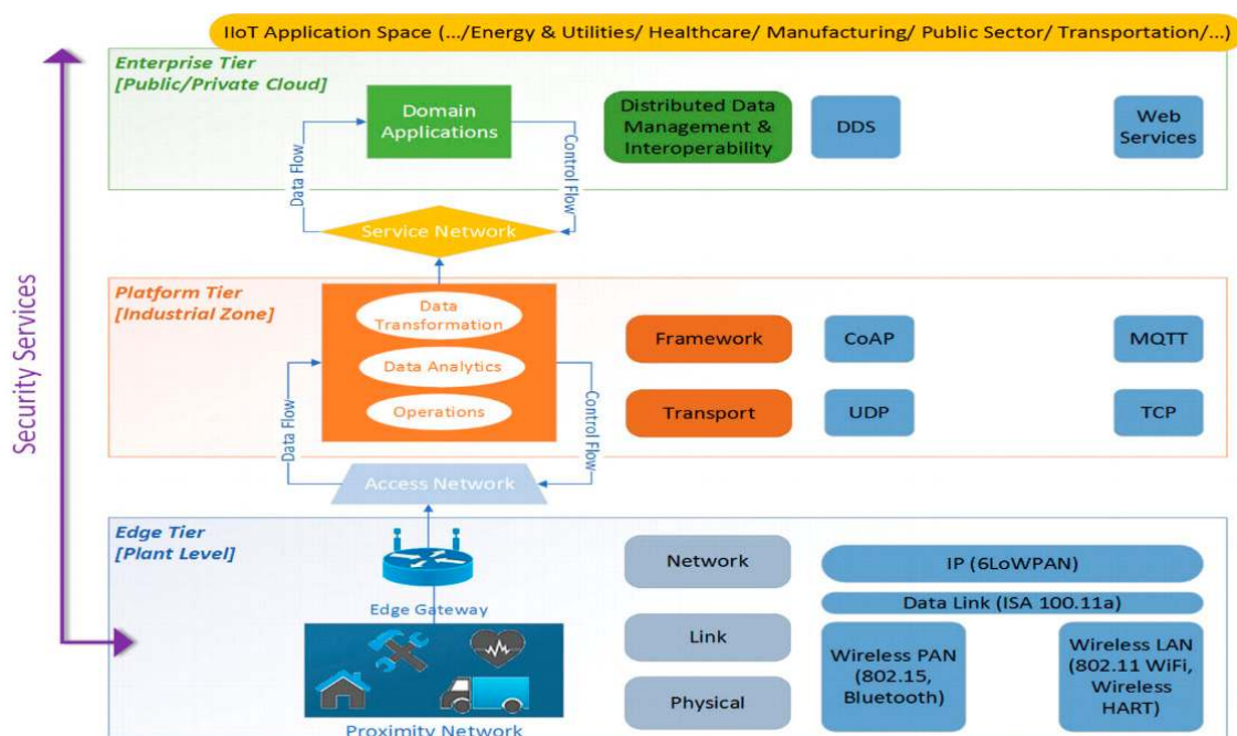
Figure 3. Three-tier architecture of IIoT connectivity and communications standards.
