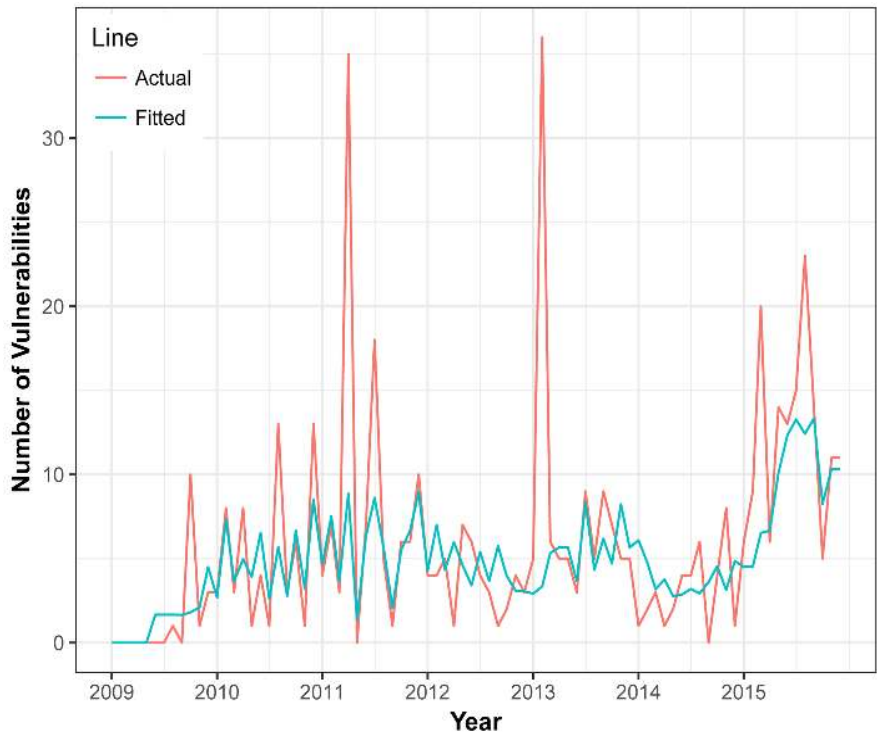
Figure 10. Original vulnerability vs. fitted vulnerabilities for windows 7 os.
