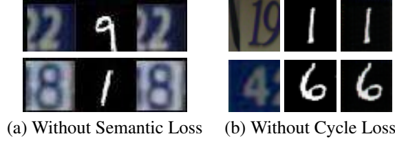
Figure 4: Ablation: Effect of Semantic or Cycle Consistency. Each triple contains the SVHN image ( left ), the image translated into MNIST style ( middle ), and the image reconstructed back into SVHN ( right ). (a) Without semantic loss, both the GAN and cycle constraints are satisfied (translated image matches MNIST style and reconstructed image matches original), but the image translated to the target domain lacks the proper semantics. (b) Without cycle loss, the reconstruction is not satisfied and though the semantic consistency leads to some successful semantic translations ( top ) there are still cases of label flipping ( bottom ).
