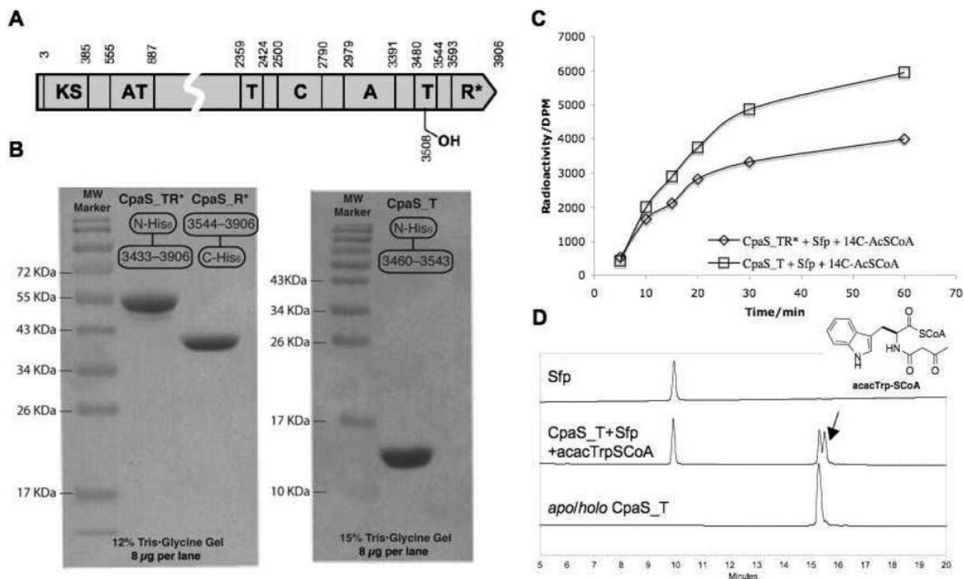
Figure 3. Overproduction of truncated CpaS proteins and their phosphopantethenylation assays. (a) Domain architecture and boundaries of CpaS (NRRL3357). (b) SDS-PAGE purity of overproduced CpaS_TR*, CpaR* and CpaS_T. (c) Phosphopantethenylation of CpaS_TR* and CpaS_T by Sfp. Time course was shown by analyzing the incorporation of [1- 14 C]acetyl-S-phosphopantetheinyl group from [1- 14 C]acetyl-CoA. (d) HPLC analysis of overproduced apolholo CpaS_T and acacTrp-S-CoA modified CpaS_T (arrow indicates N-acacTrp-S-T intermediate, predicted mass: 14625.4 Da; observed mass, 14625.0 Da)
