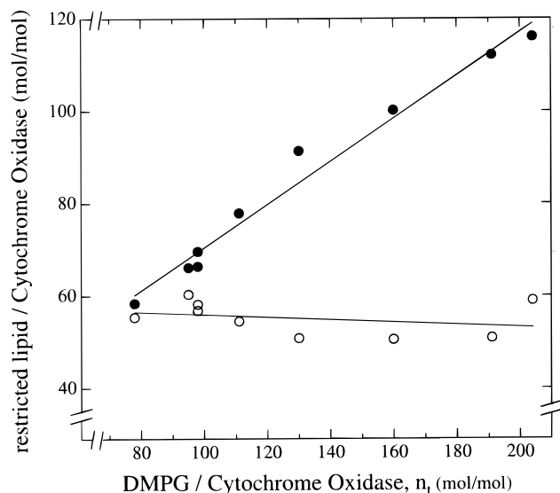
FIGURE 4: Motionally restricted lipid population in reconstituted complexes of cytochrome c oxidase with DMPG, in the absence (open circles) and in the presence (filled circles) of bound cytochrome c , as a function of the lipid/cytochrome c oxidase ratio, n_l . Stoichiometries, N_b \equiv fn_l , of motionally restricted lipid per cytochrome c oxidase monomer were calculated assuming equivalence between 14-PGSL and DMPG (i.e., K_f \approx 1 in the absence of cytochrome c ).
