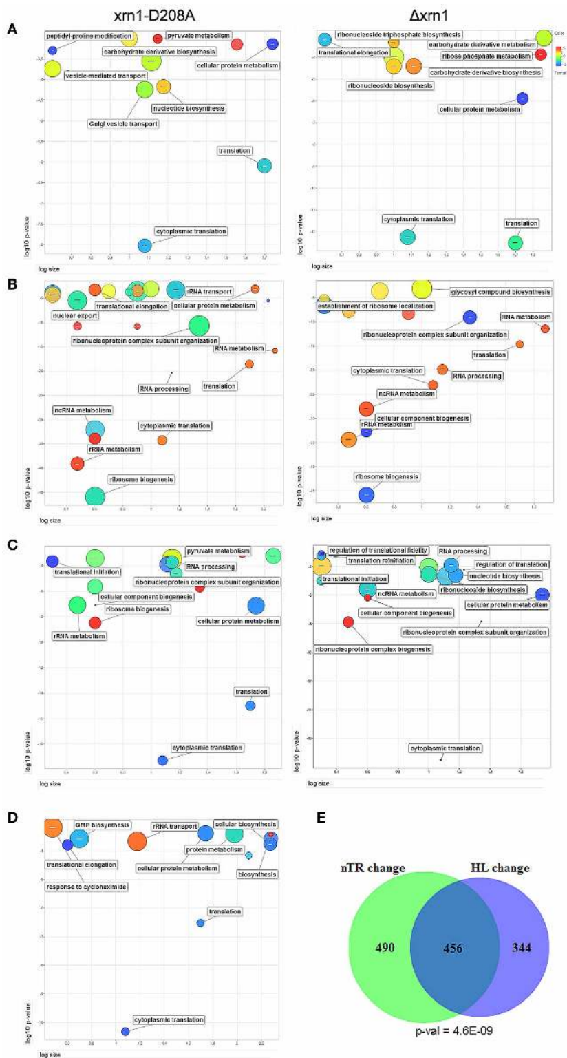
FIGURE 2 | ReVIGO plots of the GO searches. Plots of the statistically overrepresented GOs among genes in the highest 20% change in the mutant against wt in the thiolatin HL determination (A) or nTR (B) . A similar search for the genes with responsiveness \geq 8 (C) and the genes bound by Xrn1 (D) . ReVIGO plots use previous GOrilla results for the Biological Process and plot the GO categories according to their p -value
