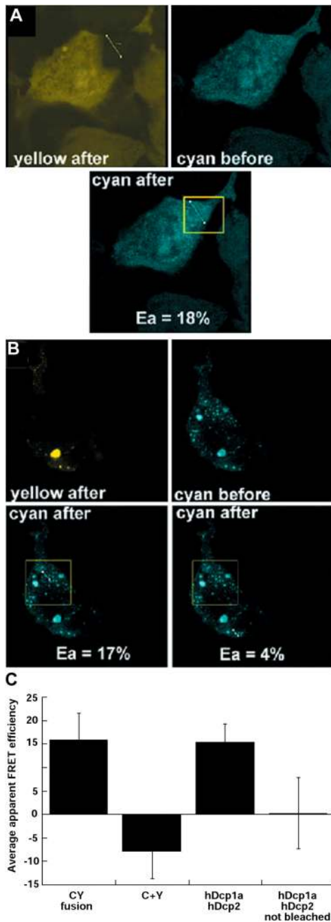
Figure 4. hDcp1a and hDcp2 interact in cytoplasmic foci. (A) Example of a FRET experiment where a fusion protein, CFP-YFP, was expressed in HEK293 cells as a positive control. A picture of the YFP signal was taken after photobleaching of a rectangular sector overlapping the cell (outlined in the CFP signal picture, bottom). A picture of the CFP signal was taken before (top right) and after (bottom) photobleaching of the YFP. Apparent FRET efficiency (18% for this experiment) was calculated as described in Materials and methods. (B) Example of a FRET experiment where CFP-hDcp1a and YFP-hDcp2 were expressed in HEK293 cells. Pictures were taken as described in A. Quantification of a foci in the bleached region shows an apparent FRET efficiency of 17% for this experiment (bottom left), whereas quantification of a foci out of the bleached region shows FRET efficiency of 4% (bottom right). (C) Histogram representing the average apparent FRET efficiency for the different constructions in different experiments. Error bars indicate the standard deviation from the independent measurements.
