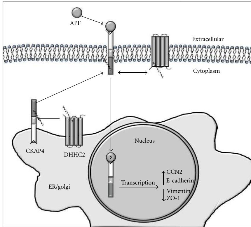
FIGURE 2: DHHC2 palmitoylation of CKAP4 is necessary for APF-mediated signaling. APF is a sialoglycopeptide that inhibits cellular proliferation of bladder epithelial cells (normal and carcinoma) and is capable of binding to the transmembrane protein CKAP4 [11, 28]. The APF/CKAP4 interaction has been shown to be required for APF's inhibition of cellular proliferation and for the alteration of specific gene expression, including E-cadherin, ZO-1, vimentin, p53, and CCN2 [11, 29]. Further, these APF-mediated changes in cellular proliferation and gene expression are regulated by DHHC2-mediated palmitoylation of CKAP4, as CKAP4 must be palmitoylated to traffic to the cell surface [22]. There is a marked increase in the nuclear abundance of CKAP4 in response to APF; however, it is not known whether APF is also present in the nucleus.
