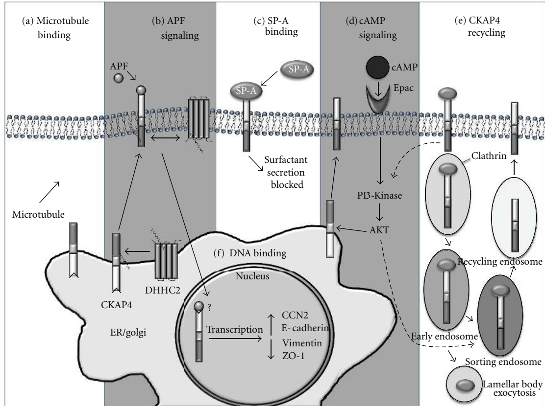
FIGURE 3: Model of CKAP4's functions at the plasma membrane, ER, and nucleus. (a) CKAP4 has been determined to be able to bind the ER to microtubules and is suspected of stabilizing the ER and/or stabilizing microtubules [6]. (b) The palmitoylation of CKAP4 by DHHC2 has been shown to be required for APF mediated signaling [14, 22]. (c) The binding of SP-A to CKAP4 inhibits the secretion of surfactant [12]. (d) An interaction between cAMP and Epac causes a signal cascade stimulating PI3-Kinase which in turn activates Akt and increases the transport of CKAP4 from the ER to the plasma membrane [18]. (e) The SP-A/CKAP4 interaction is recycled via a clathrin pathway and is stimulated by the cAMP signaling cascade [18]. (f) CKAP4 binds to the CCN2 promoter via its C-terminal domain (residues 126–501 which includes the bZIP-like DNA-binding domain) in an APF-dependent fashion [13]. It is not known whether APF binds CKAP4 in the nucleus.
