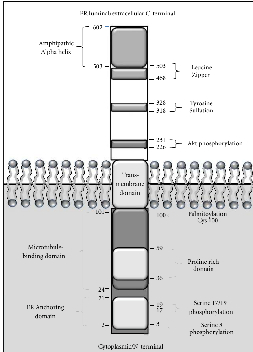
FIGURE 1: CKAP4 structural domains. CKAP4 is a 63-kDa nonglycosylated type II transmembrane protein that is phosphorylated and palmitoylated. The C-terminus is 447 amino acids long and is located in either the lumen of the ER or extracellular space, depending on the localization of the protein. It contains an alpha helical region (503–602) and a leucine zipper (468–503), which are important for oligomerization and are characteristic of the bZIP DNA-binding motif [9, 19]. Additionally, the C-terminus also contains the sites for tyrosine sulfation and Akt phosphorylation. The N-terminus is 106 amino acids long and is located in the cytoplasm. It is comprised of two major domains the microtubule binding domain and the ER anchoring domain. The microtubule-binding domain contains the site of palmitoylation (Cys 100 ) which is important for the trafficking of the protein to the plasma membrane and a proline rich sequence (36–59), whereas the ER anchoring domain has three serine residues (3, 7, and 19) which are required for phosphorylation-dependent binding to microtubules and nuclear translocation in response to APF.
