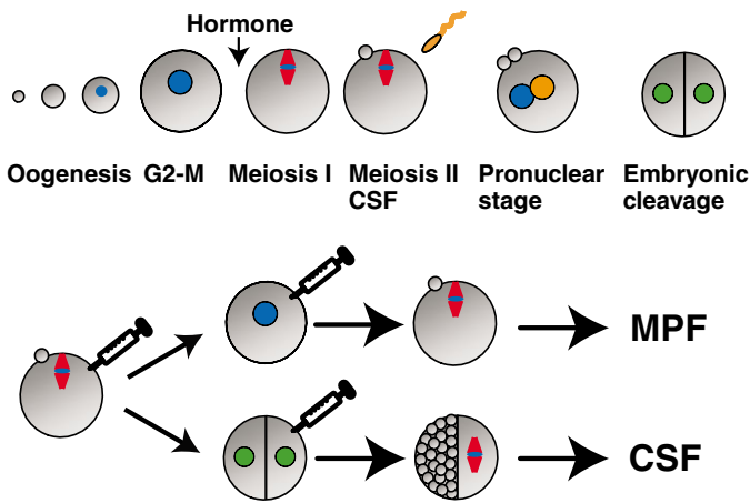
Fig. 1. MPF and CSF are key activities in vertebrate oocytes. The upper panel summarizes stages important for oocyte development and the onset of embryonic development. Oogenesis leads to the production of an immature oocyte arrested in prophase of meiosis I. After resumption of meiosis in response to hormonal stimulation, the oocyte progresses until the second arrest point in meiosis II (CSF arrest). Fertilization releases the oocyte from this arrest and triggers exit from meiosis II. The lower panel shows a simplified scheme illustrating the cytoplasmic injection experiments that led to the identification of MPF and CSF in frog oocytes. Small amounts of cytoplasm taken from mature oocytes were injected into immature oocytes or one blastomere of two-cell embryos. After injection immature oocytes resume meiosis whereas injected blastomeres arrest in metaphase. These observations led Masui and Markert to postulate that cytoplasm of mature oocytes contains two distinct biochemical activities, MPF and CSF, that regulate the oocyte maturation process (Masui and Markert, 1971).
