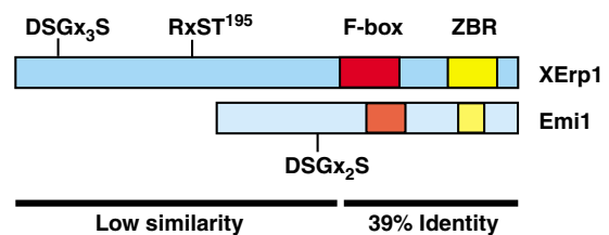
Fig. 2. XErp1 and Xenopus Emi1. Domains and positions of amino acid sequences are depicted approximately to scale. XErp1/Emi2 and Xenopus Emi1 share 39% identity in their C-terminal domains. The C-terminus of both proteins contains the F-box followed by a zinc-binding region (ZBR). Note that the XErp1 N-terminal extension is not shared by Emi1.
