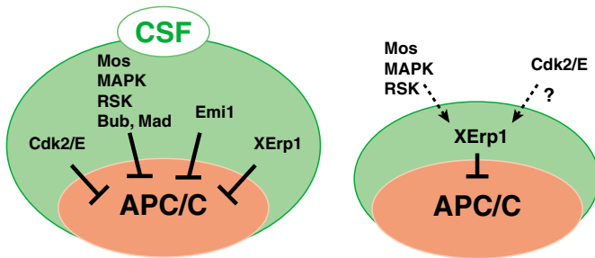
Fig. 4. Models of CSF arrest. The establishment and maintenance of CSF may involve many different, seemingly parallel pathways (left panel). However, we speculate that future investigation and reinvestigation of all proposed components could lead to a more straight-forward model in which all pathways converge onto the APC/C inhibitor Erp1 (right panel).
