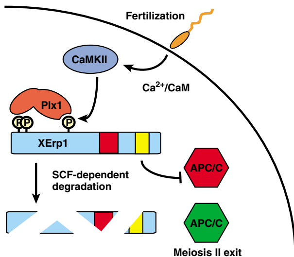
Fig. 3. Model for meiosis II exit after fertilization-induced destruction of XErp1. During CSF arrest, the APC/C is kept inactive by XErp1. Fertilization leads to the production of intracellular Ca 2+ transients that activate CaMKII. CaMKII phosphorylation on Thr195 directs Plx1 to its substrate XErp1. Plx1 phosphorylation then triggers SCF B-TRCP -dependent degradation of XErp1 by the ubiquitin/proteasome system. As a result, the APC/C is liberated from its repression and triggers meiosis II exit.
