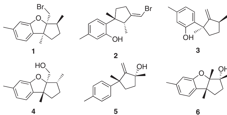
Figure 1 Chemical structures of the known sesquiterpenes isolated from Laurencia pacifica in this work. Isoaplysin (1), isolaurenisol (2), debromoisolaurinterol (3), debromoaplysinol (4), laur-11-en-10-ol (5), and 10 \alpha -hydroxydebromoepiaplysin (6).
