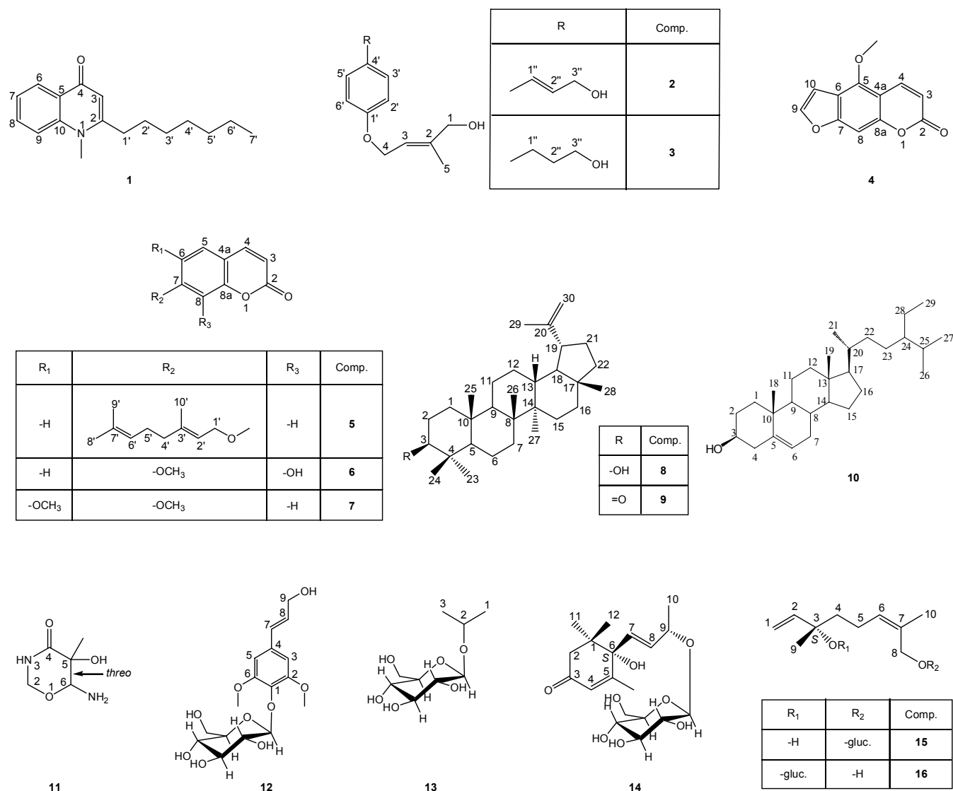
Figure 1. Structures of compounds isolated from methylene chloride ( 1 ~ 10 ) and butanol ( 11 ~ 16 ) fractions of Z. schinifolium .
