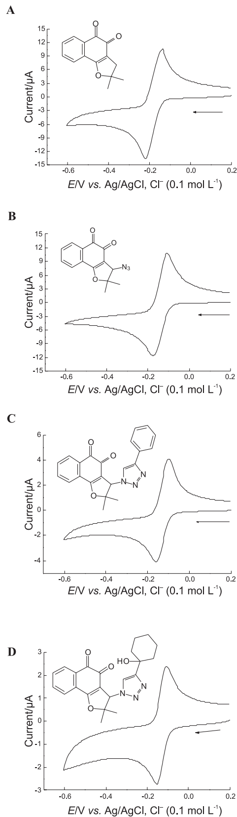
Figure 2. Cyclic voltammograms of naphthoquinones ( c = 1\text{ mmol L}^{-1} ) in buffered acetate solutions, pH 4.5, vitreous carbon electrode, E/\text{V vs. Ag/AgCl}, \text{Cl}^- ( 0.1\text{ mol L}^{-1} ). A: compound 2a , B: compound 5 , C: compound 6 and D: compound 9 .
