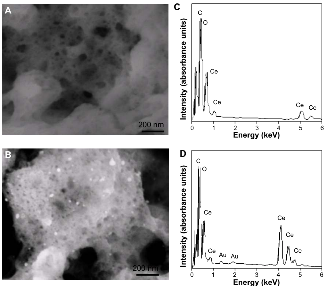
Figure 2 Scanning electron microscopic images of \text{CeO}_2 NPs (A) and \text{Au/CeO}_2 NPs (B) along with their corresponding energy dispersive X-ray spectra (C, D). Abbreviations: Au, gold; Ce, cerium oxide; \text{CeO}_2 , cerium oxide; \text{Au/CeO}_2 , gold-coated cerium oxide.
