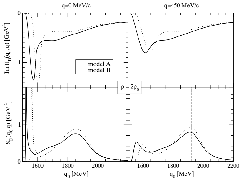
FIG. 8. The same as described in the legend to Fig. 7 for nuclear matter density \rho = 2\rho_0 .
