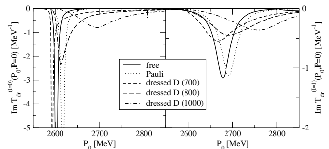
FIG. 2. Imaginary part of the in-medium DN amplitude at total momentum \vec{P} = 0 as a function of total energy P_0 for I = 0 (left panel) and I = 1 (right panel). The free amplitude in the dimensional regularization scheme of Fig. 1 (solid lines) is modified by medium corrections calculated according to Eq. (11) with various values of the cutoff: 700 MeV (short-dashed lines), 800 MeV (long-dashed lines), and 1000 MeV (dot-dashed lines). The dependence of the corrections on the cutoff is evident, except when one only considers Pauli blocking (dotted line) where the correction affects only loop momenta up to p_F = 270 MeV, well below any of the cut-off values explored.
