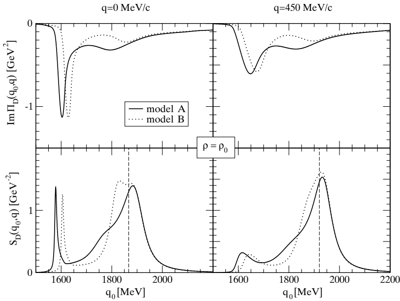
FIG. 7. Imaginary part of the D -meson self-energy (upper panels) and corresponding D -meson spectral function (lower panels) as functions of energy for two values of the meson momentum, q = 0 and q = 450 MeV at normal nuclear matter density. Results are shown for model A (solid lines) and model B (dotted lines). Thin vertical lines display the location of the D -meson pole in free space.
