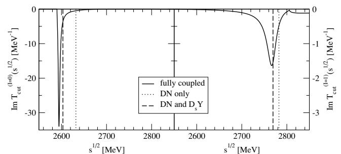
FIG. 4. Imaginary part of the DN amplitude as a function of \sqrt{s} for I = 0 (left panel) and I = 1 (right panel) obtained by using the cut-off scheme (model A).
