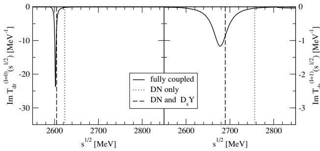
FIG. 1. Imaginary part of the DN amplitude in the dimensional regularization scheme as a function of \sqrt{s} for I = 0 (left panel) and I = 1 (right panel).
