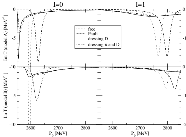
FIG. 5. Imaginary part of the in-medium DN amplitude for total momentum P = 0 as a function of the total energy P_0 for I = 0 (left panels) and I = 1 (right panels), obtained in the cut-off scheme using model A (upper panels) and model B (lower panels).
