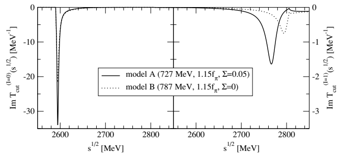
FIG. 3. Imaginary part of the DN amplitude as a function of \sqrt{s} for I = 0 (left panel) and I = 1 (right panel), obtained by using the cut-off scheme with model A (solid lines) and model B (dotted lines).
