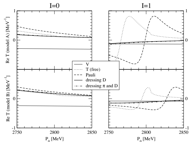
FIG. 6. Real part of the in-medium DN amplitude for total momentum \vec{P} = 0 as a function of total energy P_0 for I = 0 (left panels) and I = 1 (right panels) obtained in the cut-off scheme with model A (upper panels) and model B (lower panels). The selected range of energies covers values around the DN threshold.
