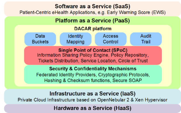
Fig. 1. Conceptual structure of the DACAR platform
