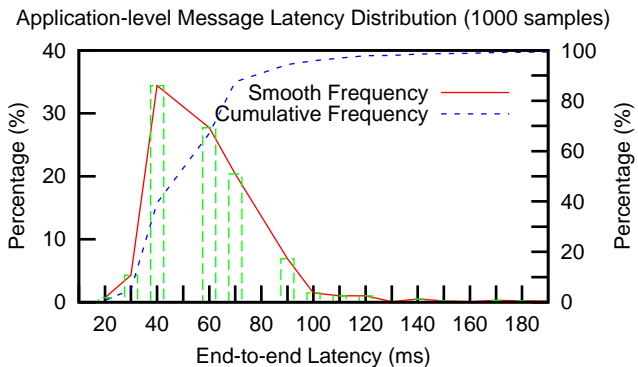
Fig. 4. Application-level message latency distribution analysis
