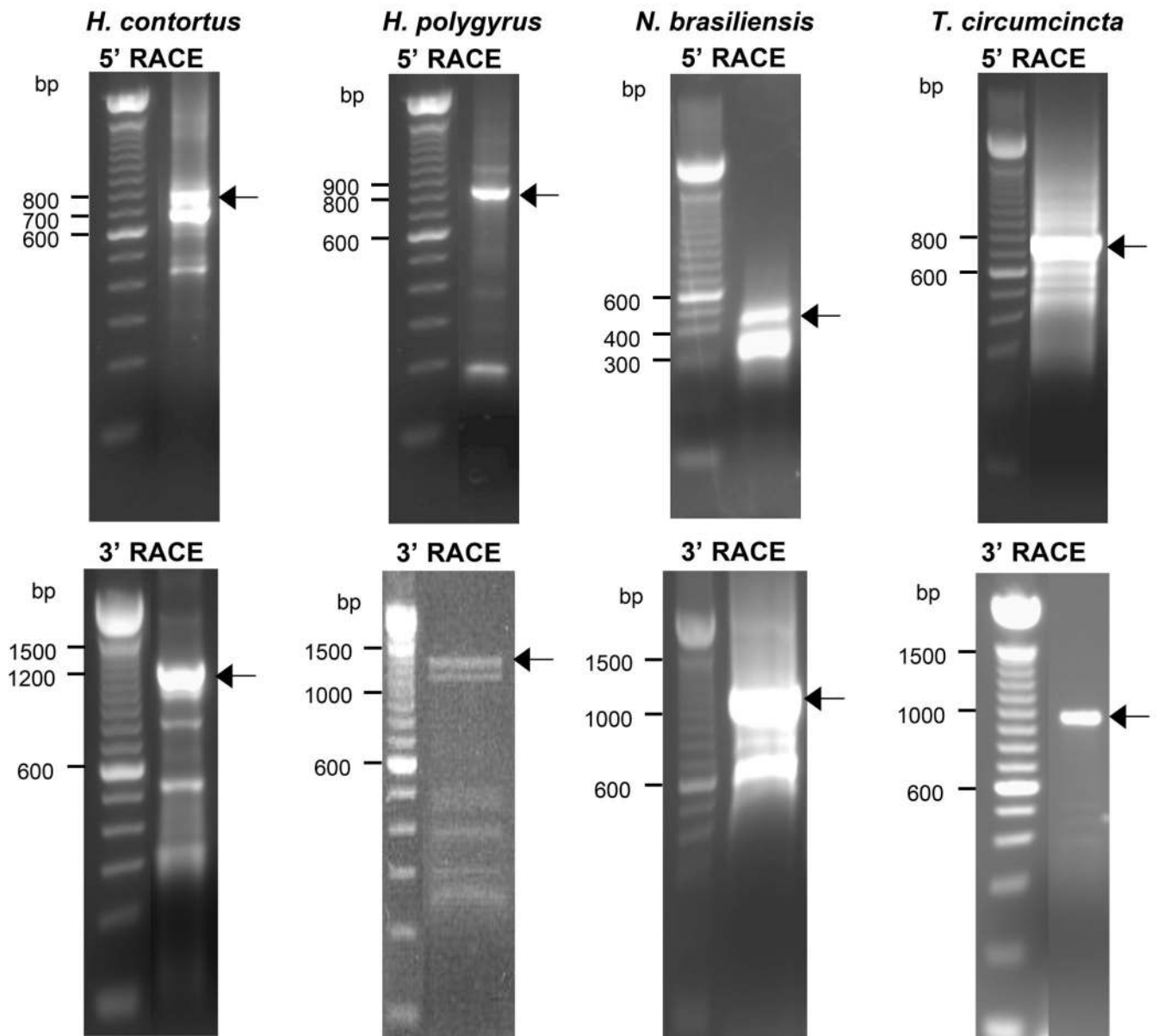
Figure 2. 5' and 3' RACE products of TGF- \beta homologues
