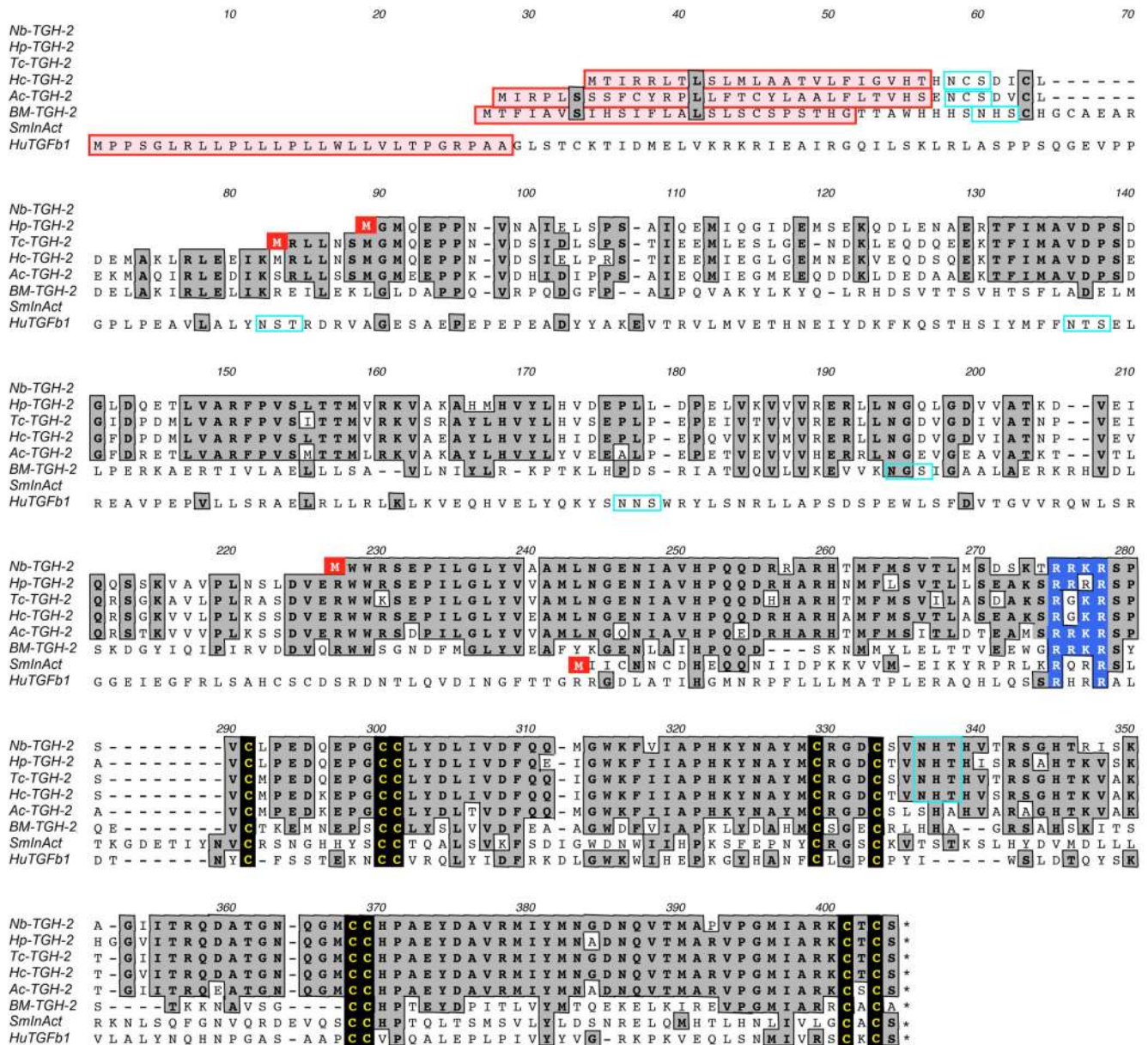
Figure 3. Full amino acid sequences and alignment of TGF-β homologues Protein alignments of known TGF-β homologues from Homo sapiens , B. malayi , A. caninum , and novel TGF-β homologues from H. contortus , H. polygyrus , N. brasiliensis and T. circumcincta . Numbering corresponds to the human protein sequence. Predicted signal sequences are shown in red boxes, or where no signal sequence is predicted, start methionines are indicated in solid red boxes. Solid blue box indicates tetrabasic protease cleavage site, yellow boxes indicate conserved cysteines. Open turquoise boxes denote potential N-glycosylation motifs (N-X-S/T). Accession numbers for novel sequences are: Hp-tgh-2 FJ410912, Nb-tgh-2 FJ410912 and Tc-tgh-2 FJ410912.
