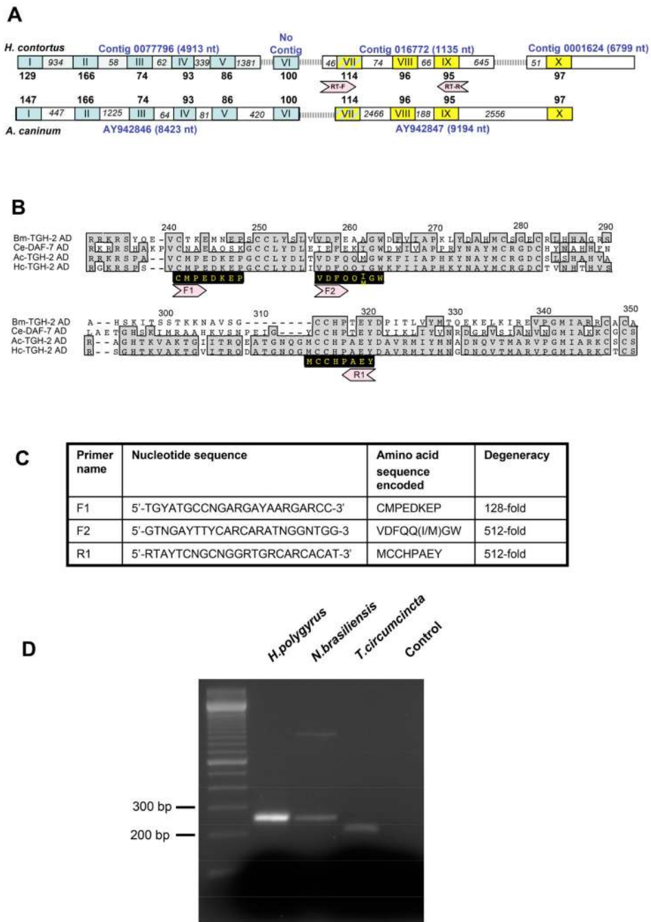
Figure 1. Primer design and amplification of tgh-2 sequences
