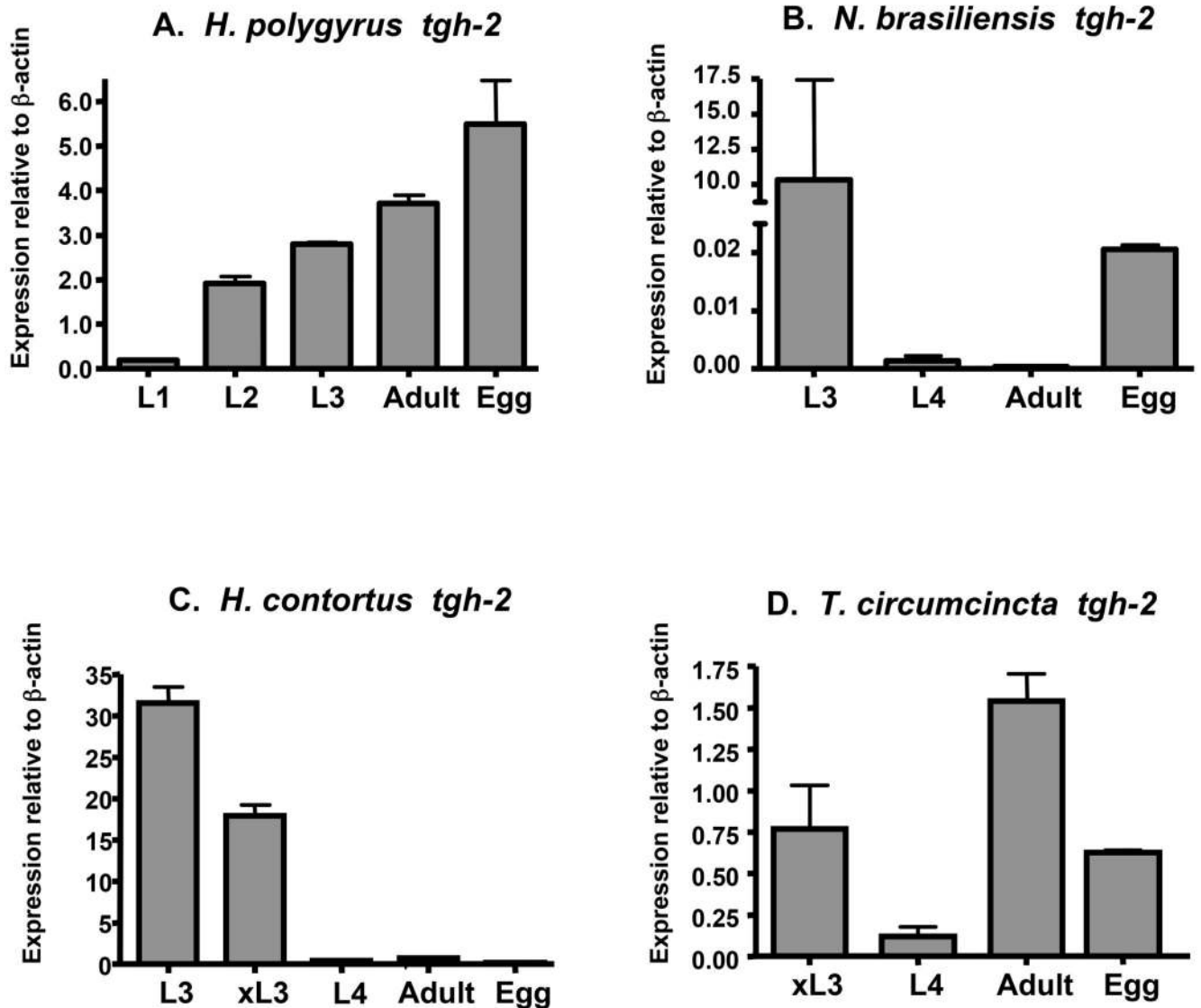
Figure 5. Expression levels of tgh-2 transcript in different life cycle stages
