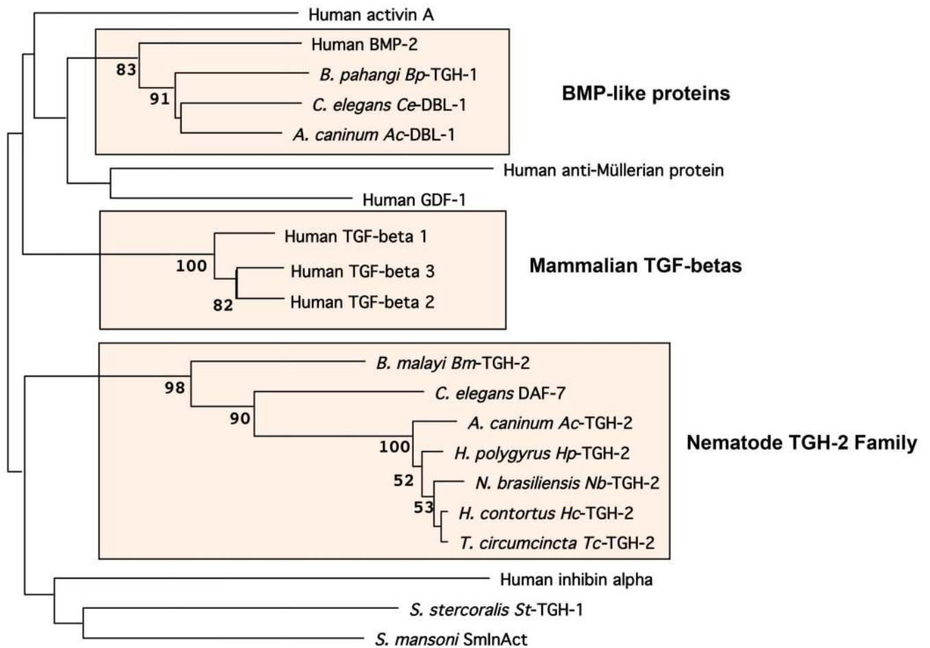
Figure 4. Phylogenetic tree of TGF- \beta superfamily members
