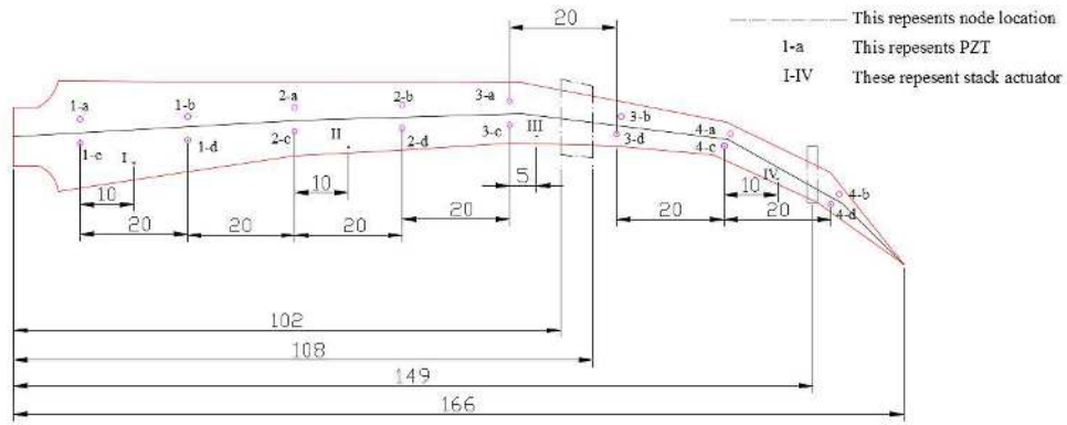
Figure 5: Schematic of the location of the sensors. The red circles represent the PZTs. The Roman numerals represent the stack actuators. The dash dot line areas manifest the nodal locations. The unit of length is the centimetre
