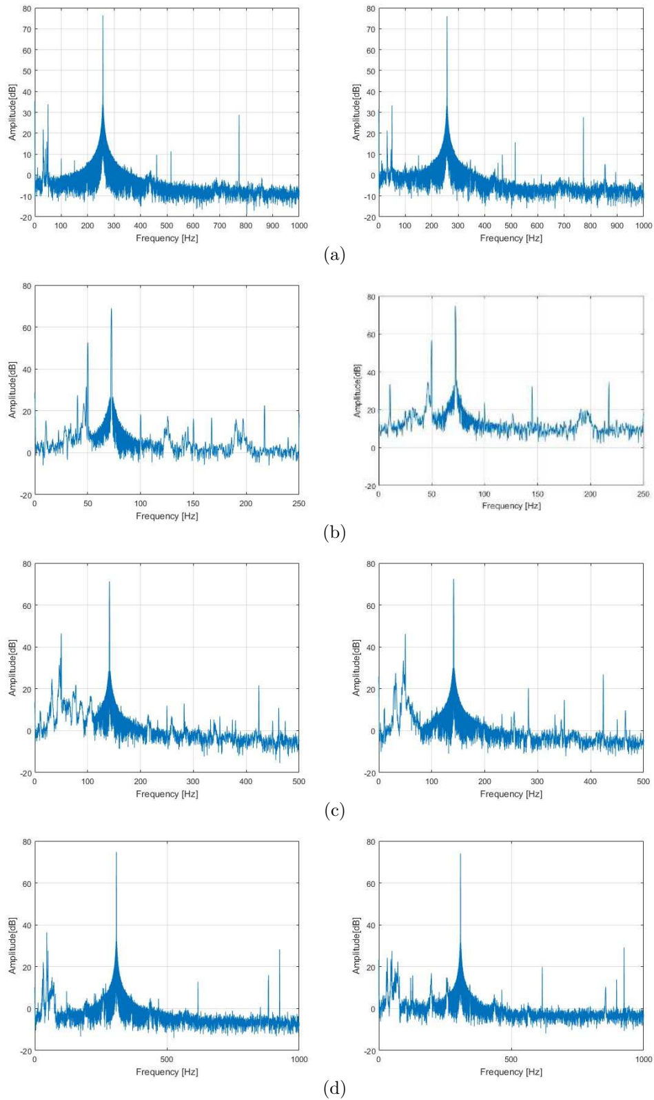
Figure 9: Power spectra density showing the fundamental peak and harmonics for the intact (left column) and impact (right column) blade excited by (a) 8 th vibration mode for Section 1, (b) 4 th vibration mode for Section 2, (c) 6 th vibration mode for Section 3 and (d) 10 th vibration mode for Section 4.
