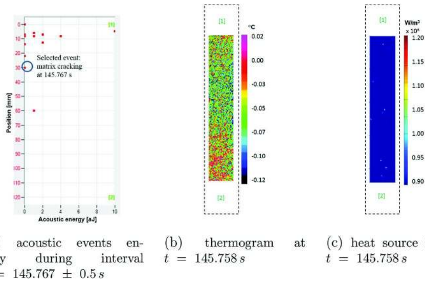
Fig. 4. Analysis of the correlation between low acoustic energy and heat source ( 0^\circ tensile test). Numbers in brackets correspond to sensors with sensor [1] (respectively [2]) positioned on the top (resp. bottom) of the specimen; vertical position of the figures fulfils the studied areas of the sample.
