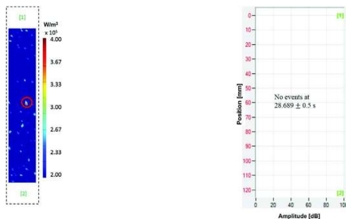
(a) heat source field at t = 28.689 \text{ s} (b) acoustic events amplitude during the interval t = 28.689 \pm 0.5 \text{ s}
