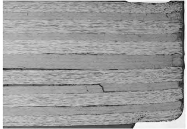
Fig. 21 Detail of the specimen struck with 50 kA, polished parallel to the 0 deg fibers in the proximity of the fastener head.
