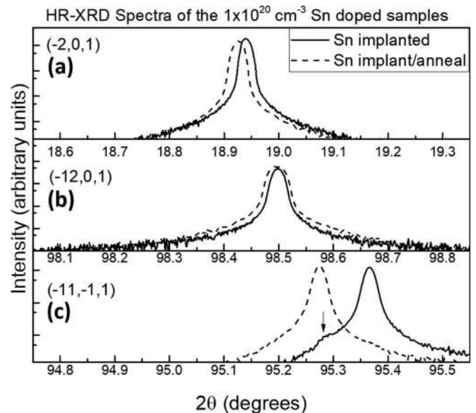
Figure 4. High resolution XRD spectra of the samples implanted with Sn to an average concentration of 10^{20} \text{ cm}^{-3} , both before and after annealing at 1150^\circ\text{C} .
