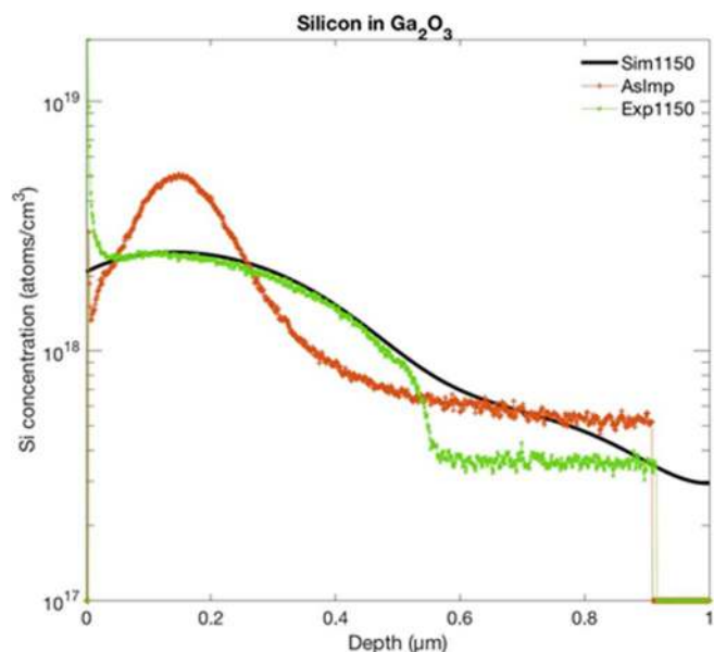
Figure 13. SIMS and simulated profiles of Si-implanted Ga 2 O 3 with a 10 18 cm -3 total dose before and after annealing at 1150°C.
