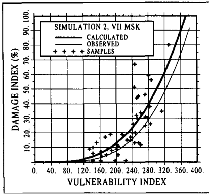
Figure 3 Second iteration in the simulation of the observed vulnerability function for intensity VII MSK and the comparison with the observed function.
