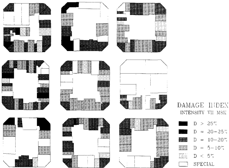
Figure 14 Damage scenario for an earthquake of intensity VII MSK.
