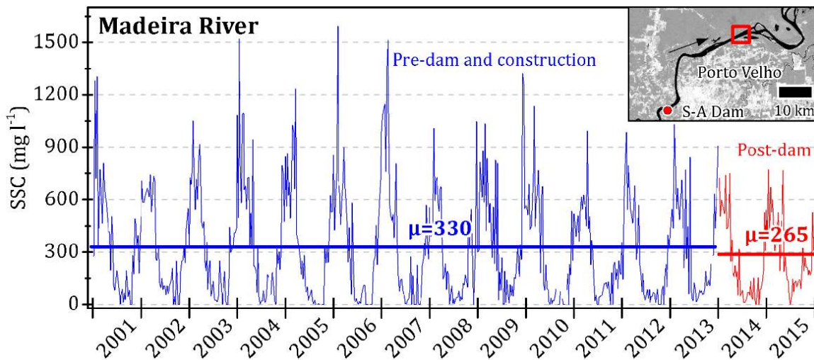
Fig. 3 Changes in surface suspended sediment concentration (SSC) in the Madeira River downstream of Santo Antônio Dam (8°48'06"S, 63°57'03"W) for pre-and post-dam construction periods. Horizontal colored lines indicate mean surface suspended sediment concentrations ( \mu ) for each period: pre-dam construction (2001-2013), and post-dam construction (2014-2015). A decrease of 20% in the mean annual SSC is detected in the Madeira River (methodological details in Supplementary Text 2). The red rectangle indicates the area used for the MODIS-SSC calibration.
