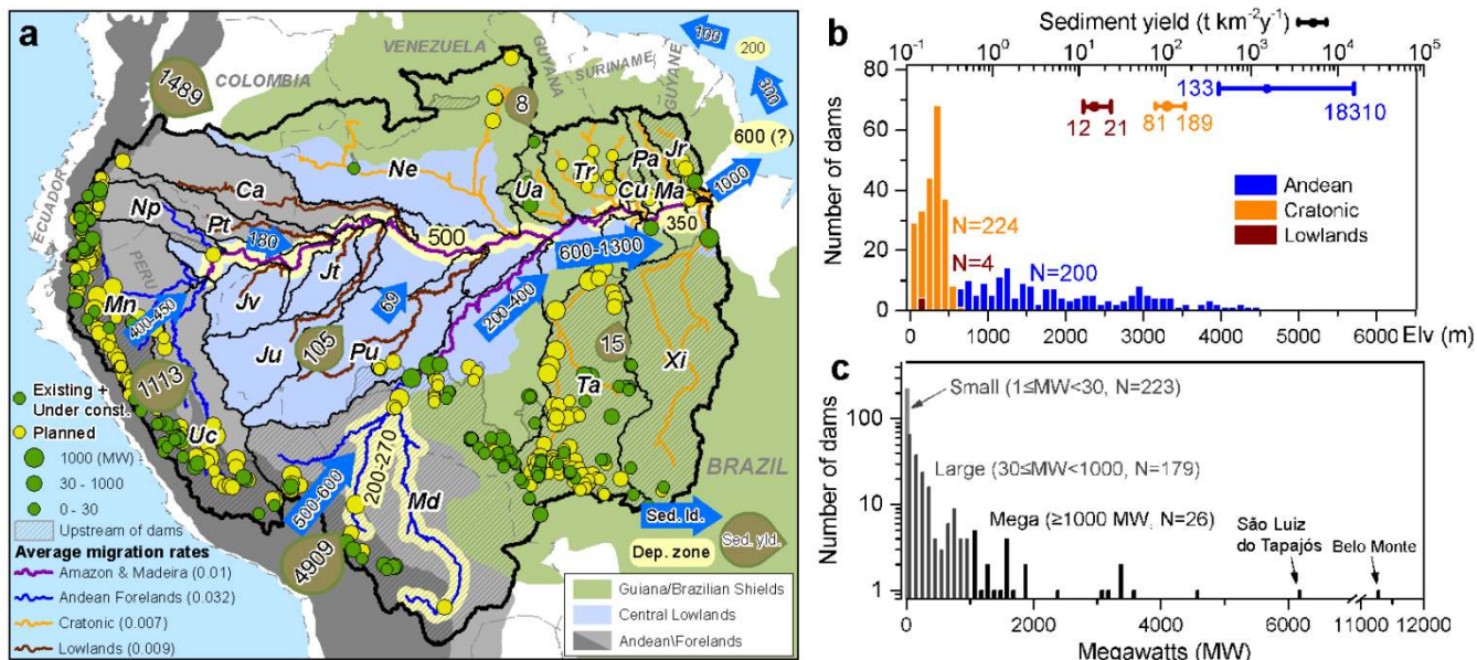
Fig. 1 The Amazon's 19 sub-basins: geologic-physiographic domains, sediments fluxes, channel migration rates and dams. (a) Andean-foreland rivers : Marañón ( Mn ), Ucayali ( Uc ), Napo ( Np ), Putumayo ( Pt ), Caqueta ( Ca ); Cratonic rivers : Jari ( Jr ), Paru ( Pa ), Curuapenema ( Cu ), Maricuru ( Ma ), Tapajós ( Ta ), Xingu ( Xi ), Trombetas ( Tr ), Negro ( Ne ), Uatumã ( Ua ); Mixed-terrain rivers : Madeira ( Md ); Lowland rivers : Juruá ( Ju ), Purús ( Pu ), Jutai ( Jt ), Javari ( Jv ). Averaged sediment yield ( \text{t km}^{-2} \text{yr}^{-1} ) for major sediment source terrains (brown balloons) 12,20 ; fluxes of sediment ( \text{Mt yr}^{-1} ) (blue arrows); major depositional zones (storage, \text{Mt yr}^{-1} ) (yellow shading) 12,18 ; Mean channel migration rates ( \text{ch-w yr}^{-1} ) by physiographic provinces 23 (red, green and blue lines) are shown. Migration rates of 0.01 were estimated for the Solimões-Amazon and Madeira rivers (purple line). (b) Numbers of dams in each elevation range (bars) and geological region (Andean, Cratonic, and Lowlands). Ranges and means of sediment yields ( \text{t km}^{-2} \text{yr}^{-1} ) measured in each region (color coded) are shown along the upper x-axis. (c) Histogram of the number of dams scaled by their hydroelectric capacity (MW).
