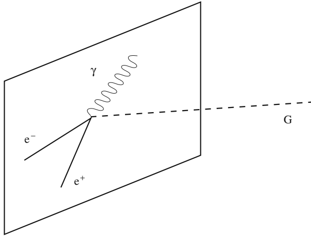
Fig. 4 The confinement of matter to the brane, while gravity propagates in the bulk (from [84])
