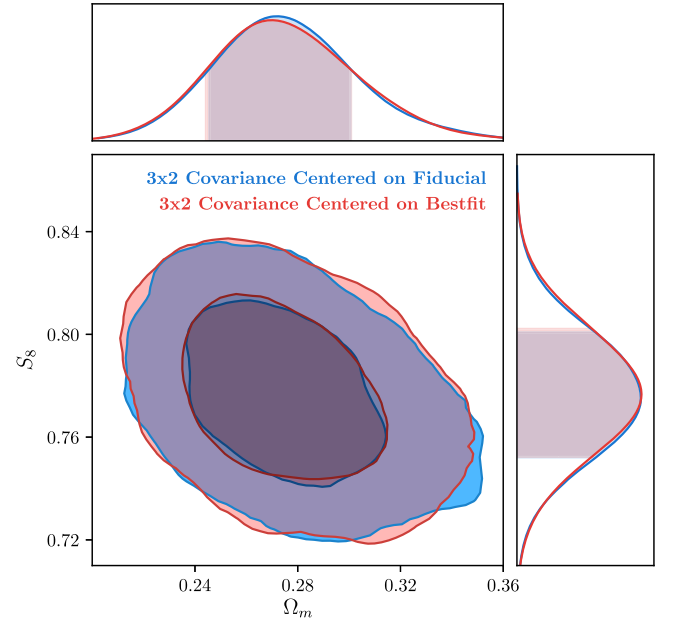
FIG. 21. Constraints on \Omega_m and S_8 using the fiducial covariance matrix and using the covariance based on the cosmological model centered on the means of the posteriors (“Bestfit”) obtained after unblinding. The two agree very well, indicating little dependence on the fiducial model assumed for the covariance.
