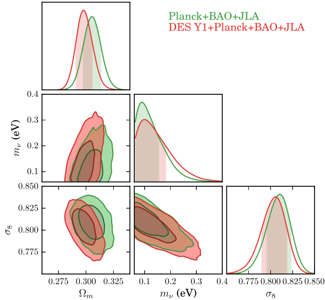
FIG. 15. \Lambda CDM constraints on the sum of the neutrino masses from DES and other experiments. The lower power observed in DES can be accommodated either by lowering \Omega or \sigma_8 or by increasing the sum of the neutrino masses.
