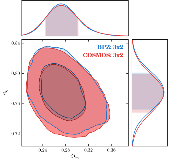
FIG. 20. Constraints on \Omega_m and S_8 when using the shifted BPZ redshift distributions as the default for n_s^l(z) , compared with those obtained when using the COSMOS redshift distribution, which have different shape, as seen in Fig. 4 of Ref. [88].
