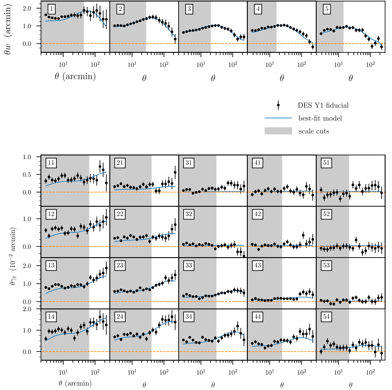
FIG. 2. Top panels: scaled angular correlation function, \theta w(\theta) , of REDMAGiC galaxies in the five redshift bins in the top panel of Fig. 1, from lowest (left) to highest redshift (right) [94]. The solid lines are predictions from the \Lambda CDM model that provides the best fit to the combined three two-point functions presented in this paper. Bottom panels: scaled galaxy-galaxy lensing signal, \theta\gamma_t (galaxy-shear correlation), measured in DES Y1 in four source redshift bins induced by lens galaxies in five REDMAGiC bins [93]. Columns represent different lens redshift bins, while rows represent different source redshift bins, so, e.g., the bin labeled 12 is the signal from the galaxies in the second source bin lensed by those in the first lens bin. The solid curves are again our best-fit \Lambda CDM prediction. In all panels, shaded areas display the angular scales that have been excluded from our cosmological analysis (see Sec. IV).
