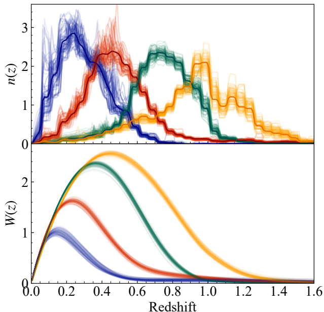
FIG. 2: Estimated redshift distributions for the weak lensing catalog, divided into four redshift bins (upper panel). Fainter lines indicate the realisations, whose spread represents the uncertainty in their estimation. Darker, solid lines denote the mean of the ensemble. These are derived using the joint SOMPZ and WZ methodology, summarised in Section III A and detailed in [82]. The stair-step appearance is an artifact of using a binned representation for the n(z) and is immaterial to the cosmological results. In the lower panel, the lensing kernel (defined in equation 14) for each of the source redshift bins demonstrates that the DES Y3 sample is most sensitive between z = 0.1 - 0.7 .
