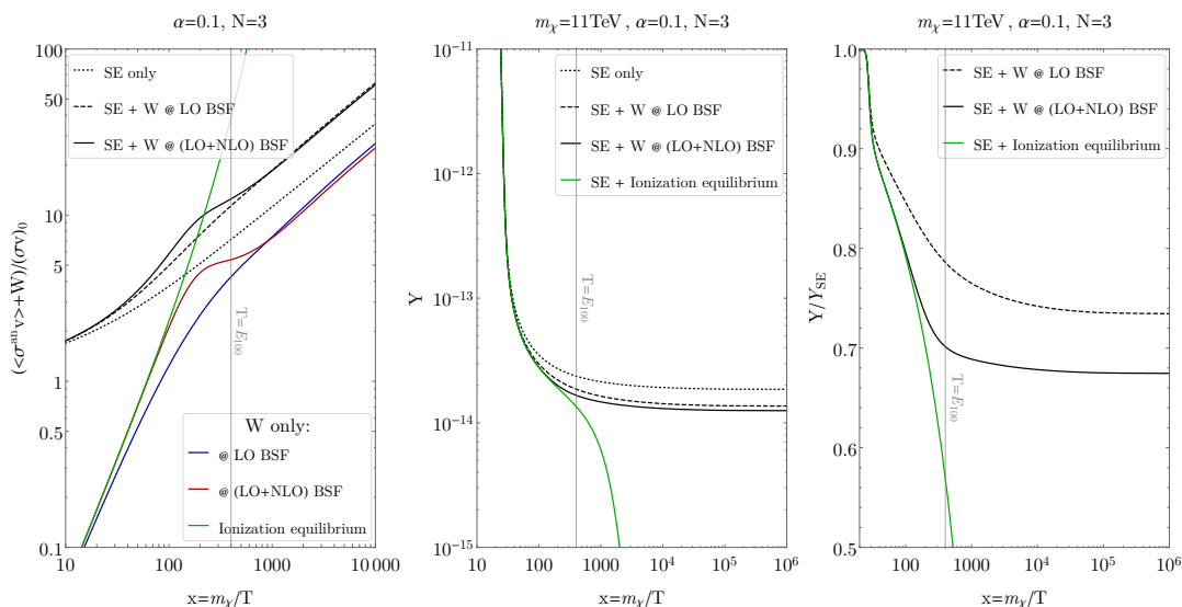
Figure 8. Impact of bound-state formation at NLO on the evolution of the thermal relic abundance. Here, Y \equiv n_\chi/s , where s is the SM entropy density, and Y_{SE} assumes Sommerfeld enhanced annihilation only.
