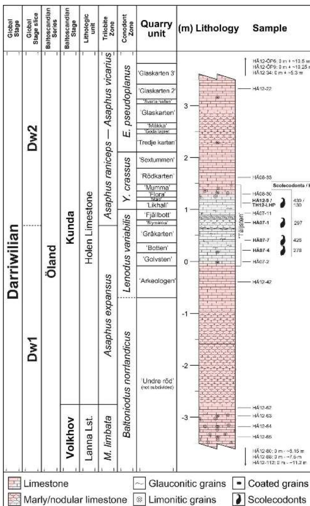
Fig. 2. Sedimentary profile of the sampled section at Hällekis (modified from Lindskog et al. 2015, with quarry units added from Schmitz 2013). All palynomorph samples are included and those yielding scolecodonts are marked with a symbol (note that sample HÄ12-64 and HÄ12-80 yielded one possible scolecodont fragment each). The abundance (number of specimens per kg of rock) is included.
