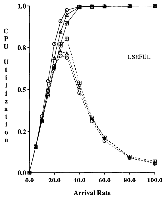
Figure 8d: CPU Utilization
