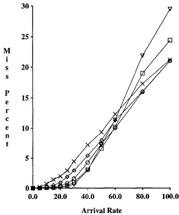
Figure 7: Data Contention
