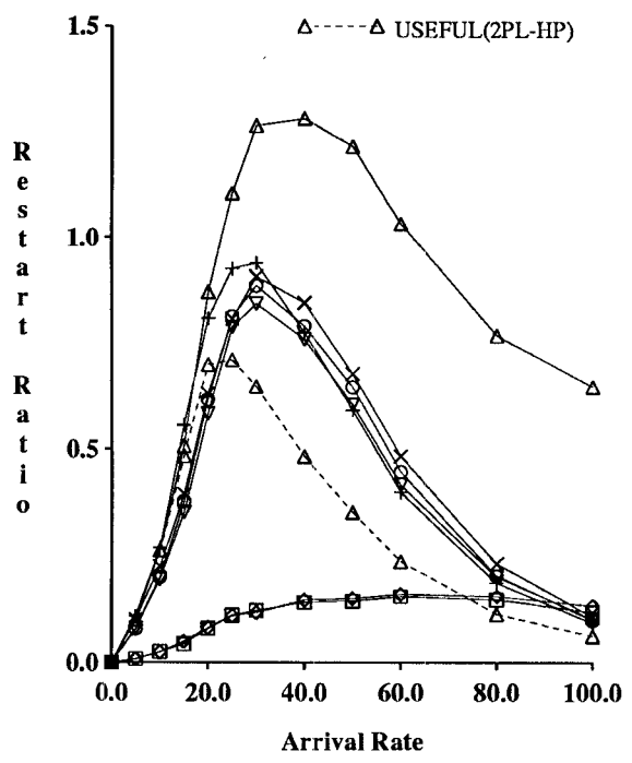
Figure 2c: Restarts (Baseline)
