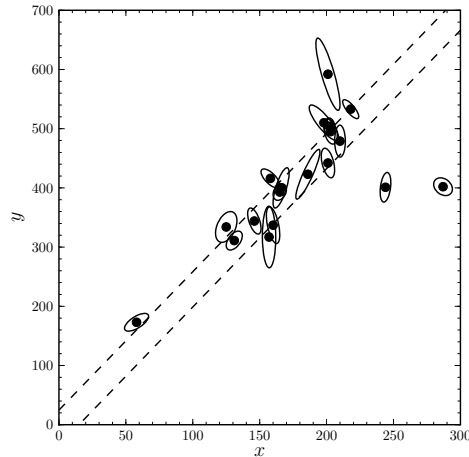
Figure 13.— Partial solution to Exercise 17: The maximum-likelihood fit, allowing for intrinsic scatter.
