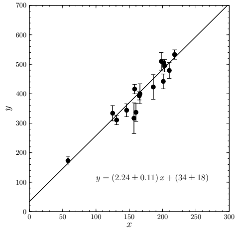
Figure 1.— Partial solution to Exercise 1: The standard weighted least-square fit.
