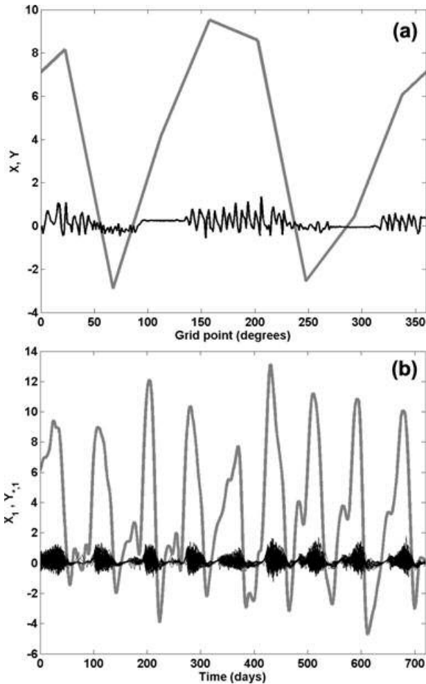
Fig. 2. (a) Snapshot of the spatial distribution of a solution at an arbitrary time. (b) Time evolution of the variables of the first cell.
