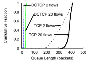
Figure 13: Queue length CDF (1Gbps)
