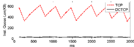
Figure 1: Queue length measured on a Broadcom Triumph switch. Two long flows are launched from distinct 1Gbps ports to a common 1Gbps port. Switch has dynamic memory management enabled, allowing flows to a common receiver to dynamically grab up to 700KB of buffer.
