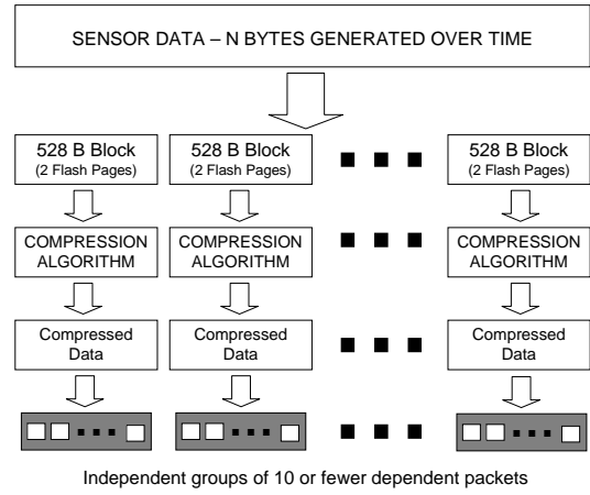
Figure 5. Data is separated into individual blocks before being compressed and divided into packets. Each packet in a shaded block cannot be decompressed without the packets that precede it, but packets in different shaded blocks are independent of one another.
