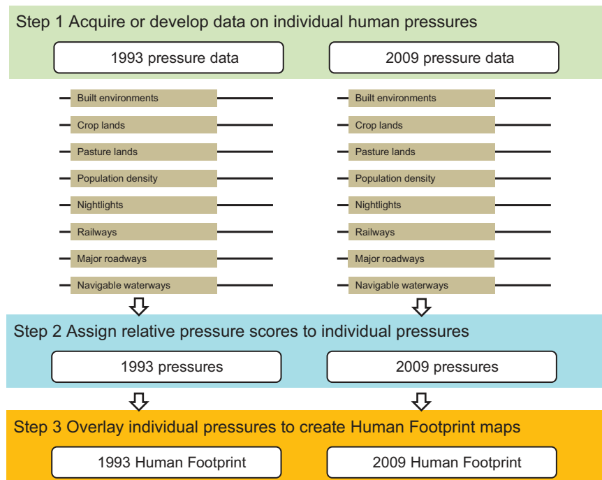
Figure 1. Workflow of the Human Footprint approach to mapping cumulative human pressures on the environment.
