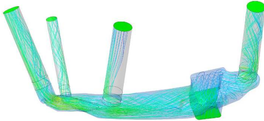
Fig. 15. A CFD simulation of the initial design.
