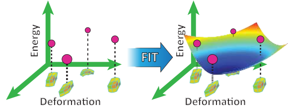
Figure 7: Metamaterial potential energy functions are fitted to the deformation-energy samples using a least-squares optimization.
