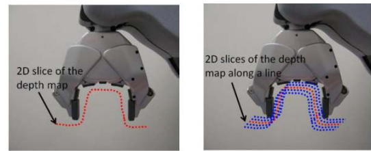
Figure 26: PR2 gripper and associated grasp pattern [34].
