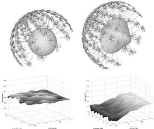
Figure 11: Top) Grasp candidates performed on SQ. Bottom) Grasp quality for each candidate [20].
