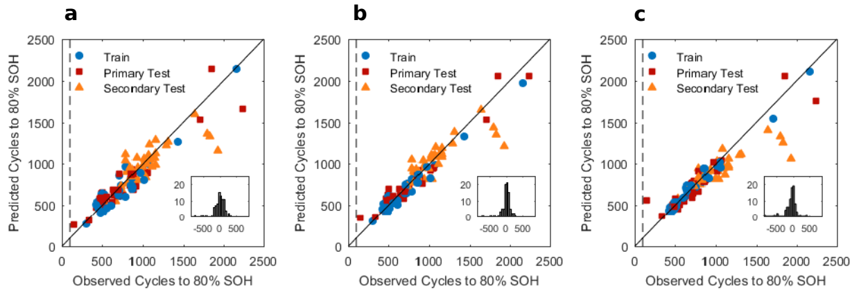
Figure 3 | Observed and predicted cycles to 80% SOH for several implementations of the feature-based model. The training data are used to learn the model structure and coefficient values. The testing data are used to assess generalizability of the model. We differentiate the primary test and secondary test datasets because the latter was generated after model development. The vertical dotted line indicates when the prediction is made in relation to the observed cycle life. The inset shows the histogram of residuals (predicted - observed) for the primary and secondary test data. a , "variance" model using only the log variance of \Delta Q_{100-10}(V) . b , "discharge" model using six features based only on discharge cycle information, described in Table 1. c , "full" model using the nine features described in Table 1. Because some temperature probes lost contact during experimentation, four cells are excluded from the full model analysis.
