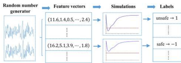
FIGURE 5. Generation of the training dataset.
